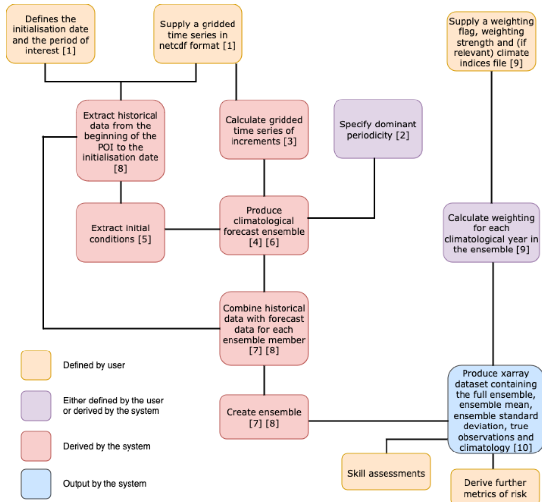
Figure 1. Flow chart showing how the General TAMSAT-ALERT implementation works. The numbers in square brackets refer to the modelling steps described in Sect. 2.1.
