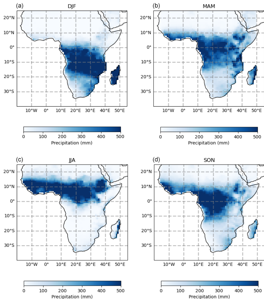
Figure 8. Seasonal cycle in precipitation over Africa: precipitation accumulations for DJF (a), MAM (b), JJA (c) and SON (d).
