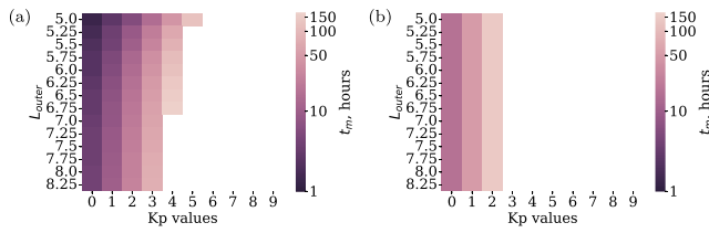
FIG. 10. Time to monotonicity t_m for L_{\text{outer}} vs Kp over a week, for Neumann (left) and Dirichlet (right) outer boundary conditions.
