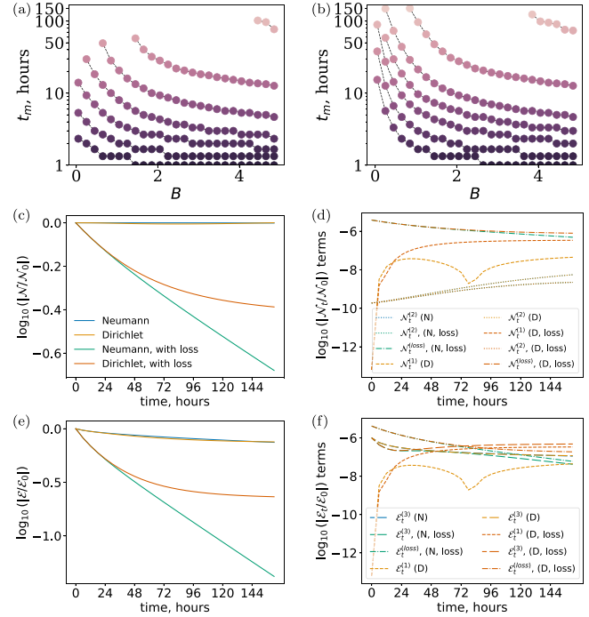
FIG. 16. Same as Fig. 6 but compares the higher step size B = 5 experiments to their equivalents with loss from pitch angle scattering. Note that the outer boundary terms \mathcal{N}_t^{(1)} , \mathcal{E}_t^{(1)} for the loss experiments represent gains as material flows into the domain.
