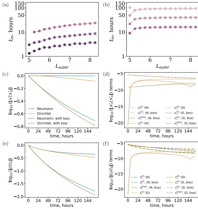
FIG. 17. Same as Fig. 16 but investigating the interaction between L_{\text{outer}} and loss, for L_{\text{outer}} = 7.5 .
