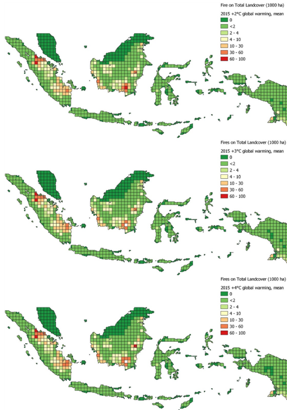
Figure 6. Total burned area for multi-model ensemble mean storyline under +2-, 3-, and 4-degrees global warming (top to bottom).
