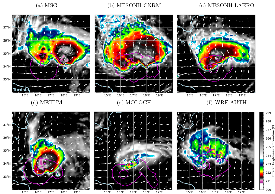
Figure 9. Infrared 10.8\mu\text{m} brightness temperature (in K, low values highlighted) observed by Meteosat Second Generation (MSG, (a)) and simulated from high-resolution model runs (b–f) in an area of intense deep convection at 00:00 UTC on 16 September. The 300 hPa wind (vectors) and MSLP (magenta contours every 5 hPa below 1010 hPa) are overlaid from the IFS analysis in panel (a) and from the high-resolution model runs in panels (b)–(f).
