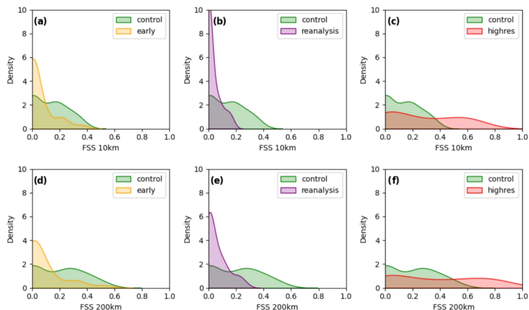
Figure 10. Fractions skill score (FSS) for the infrared 10.8\mu\text{m} brightness temperature simulated in the control and sensitivity runs and assessed against MSG's SEVIRI observations for a threshold of 223 K and scales of 10 km (a–c) and 200 km (d–f) for the sensitivity to initial time (a, d), initial data (b, e) and horizontal resolution (c, f). Probability distribution functions are computed over all grid points and from 18:00 UTC on 15 September to 06:00 UTC on 16 September every 3 h for the five models and variants illustrated in Fig. 9.
