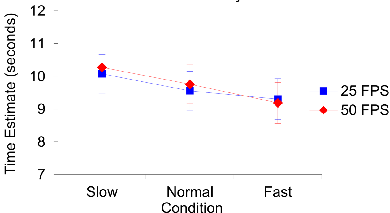
Fig 3. Illustration of the produced mean time estimates per condition and frame rate (fps). The slow 25 fps condition ( n = 10, M = 10.08, SE = 0.59 ), the slow 50 fps condition ( n = 10, M = 10.27, SE = 0.63 ), the normal 25 fps condition ( n = 10, M = 9.56, SE = 0.59 ), the normal 50 fps condition ( n = 10, M = 9.76, SE = 0.59 ), the fast 25 fps condition ( n = 8, M = 9.31, SE = 0.63 ), the fast 50 fps condition ( n = 9, M = 9.188, SE = 0.63 ). The error bars represent the standard errors of the mean in each condition.
