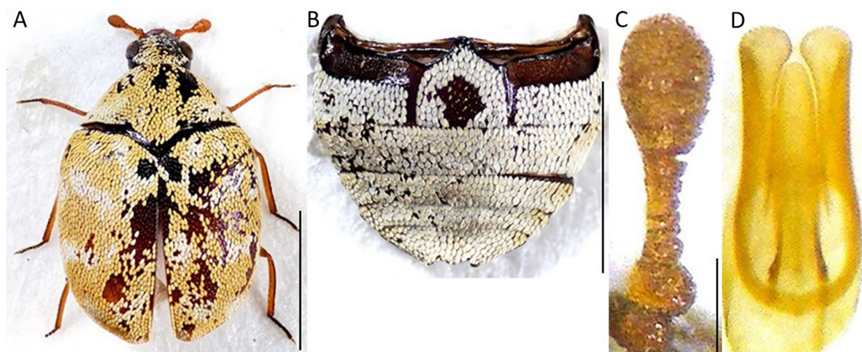
Figure 4. Anthrenus (Anthrenus) kittenbergeri . A) Habitus (scale bar = 1 mm). B) Ventrites (scale bar = 1 mm). C) Antenna (scale bar = 100 µm). D) Aedeagus (scale bar = 100 µm).
