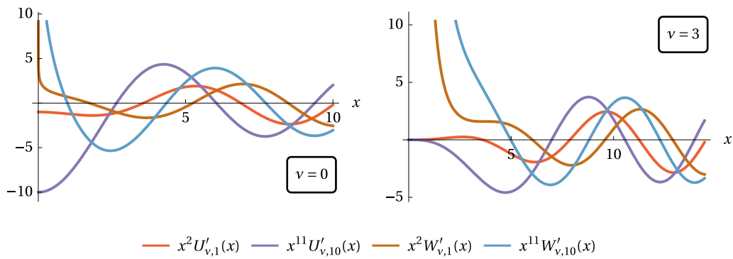
Figure 10: Plots of x^{\eta+1} U'_{v,\eta}(x) and x^{\eta+1} W'_{v,\eta}(x) .
