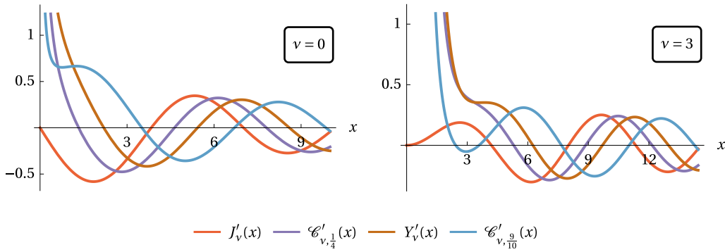
Figure 4: Plots of \mathcal{C}'_{v,\tau}(x) .
