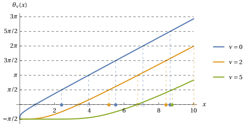
Figure 2: Plots of \theta_\nu(x) . The filled colour-coded dots on the horizontal axis indicate the positions of zeros j_{\nu,k} and the hollow dots the positions of zeros y_{\nu,k} . The phase functions are calculated using the method of [Hor7].
