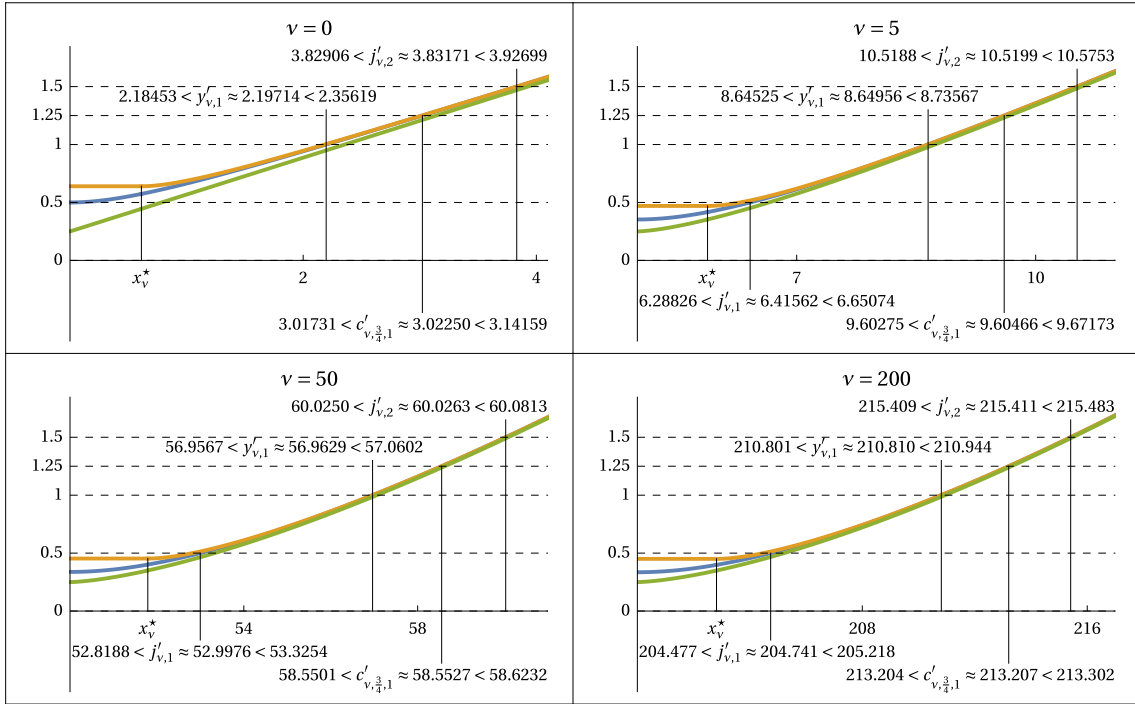
Figure 9: All plots show the scaled Bessel derivative phase function \frac{1}{\pi}\varphi_\nu(x) (blue), and its scaled bounds \frac{1}{\pi}\tilde{\varphi}_\nu(x) (orange) and \varphi_\nu(x) (green). The zeros c'_{\nu, \frac{3}{4}, 1} are the first zeros above j'_{\nu, 1} of \mathcal{C}'_{\nu, \frac{3}{4}}(x) , which up to a constant factor coincides with J'_\nu(x) - Y'_\nu(x) .
