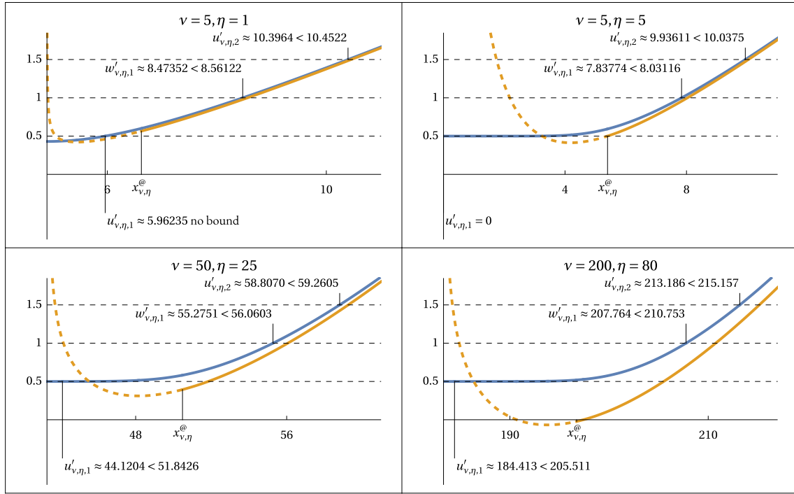
Figure 11: All plots show the scaled phase function \frac{1}{\pi}\psi_\nu(x) (blue), and its scaled bound \frac{1}{\pi}\tilde{\psi}_\nu(x) (orange). The quality of the bounds for u'_{\nu,\eta,k} and w'_{\nu,\eta,k} increases with k .
