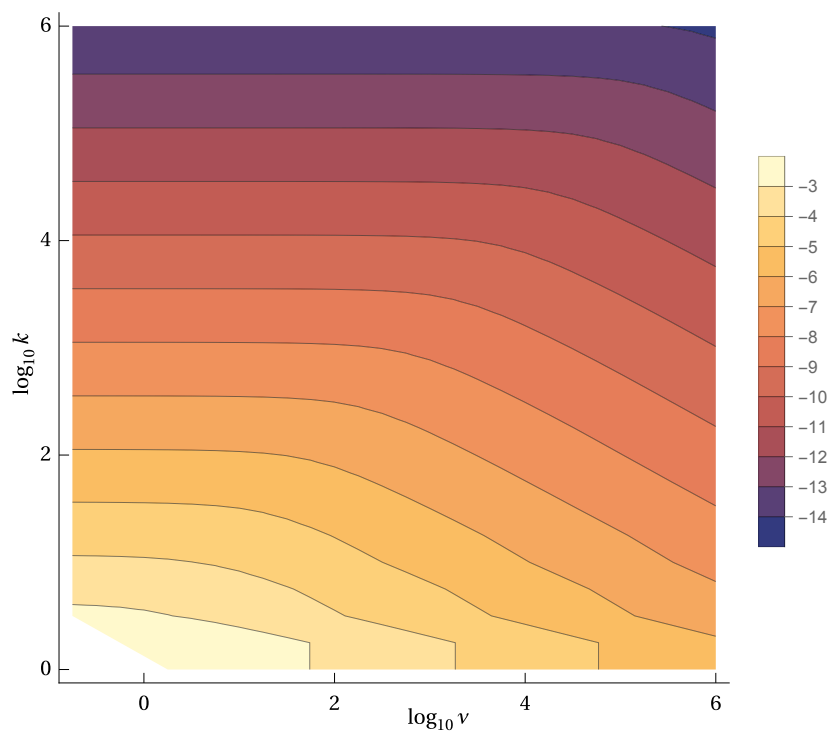
Figure 13: The contour plot of \log_{10} \left( \frac{\tilde{j}'_{v,k}}{\tilde{z}'_{v,k}} - 1 \right) , which estimates from above the maximum possible order of the relative error of our approximations of j'_{v,k} .
