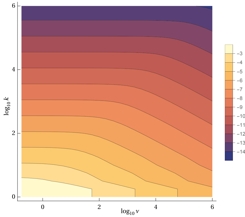
Figure 12: The contour plot of \log_{10} \left( \frac{\tilde{j}'_{v,k}}{j'_{v,k}} - 1 \right) , which estimates from above the maximum possible order of relative error of our approximations of j_{v,k} .
