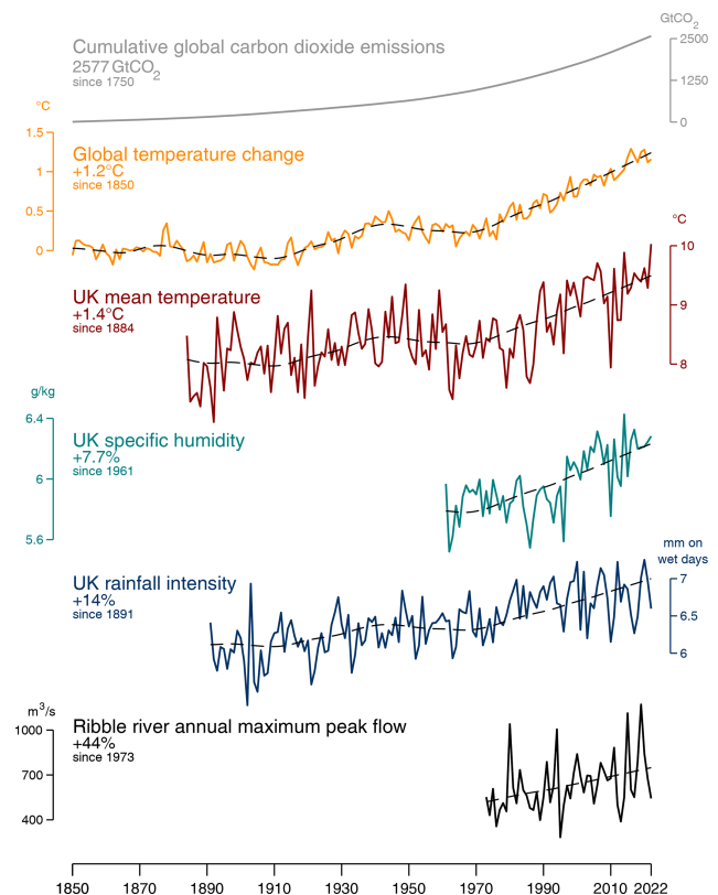
Figure 1. An observation-based causal chain from global carbon dioxide emissions to peak flow in the Ribble River. Cumulative anthropogenic global carbon dioxide emissions (grey; Friedlingstein et al., 2023) are causing global temperatures to increase (orange; the 41-year loess smoothed version in dashed black; Morice et al., 2021). Global warming is experienced locally as warmer UK temperatures (red) and increased specific humidity (green) with corresponding increases in rainfall intensity (blue) (all based on data from Hollis et al., 2019). Annual maximum peak flow on the Ribble River has increased in the last 50 years (black; NRFA, 2023). Dashed black lines show regressions onto the smoothed global temperature time series.
