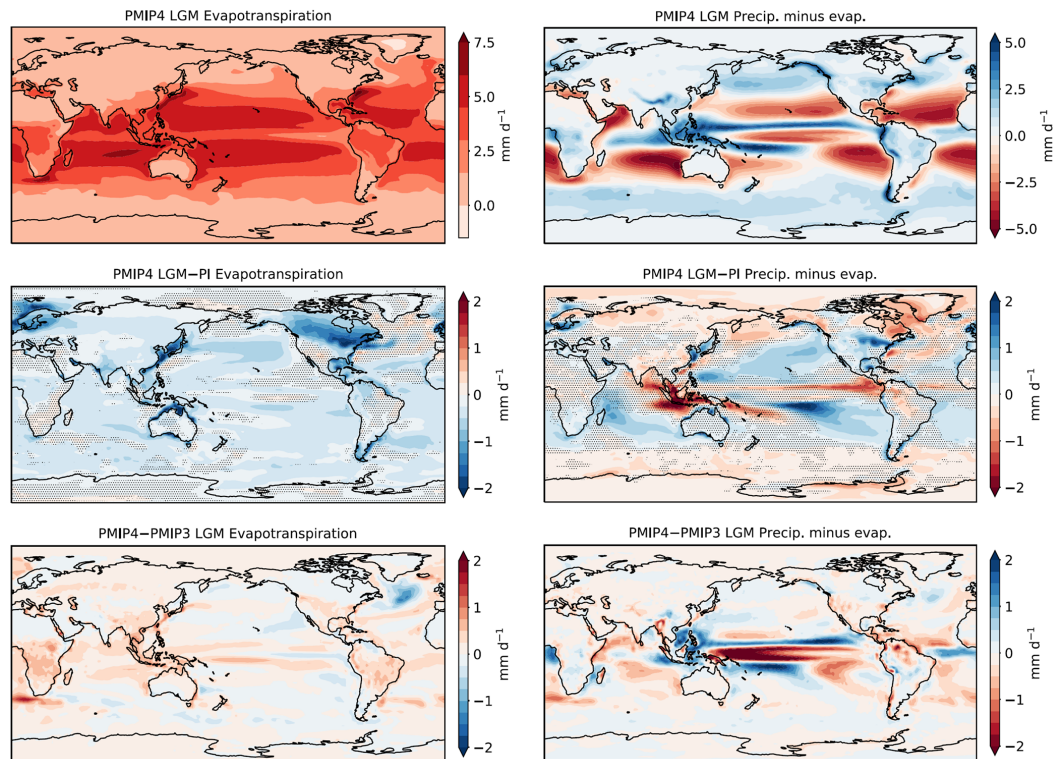
Figure 8. Same as Fig. 2 for mean annual evaporation (left-hand side) and mean annual net precipitation (precipitation–evaporation, right-hand side). All values are in mm d -1 . Stippling shows areas where less than nine models agree on the sign of change.
