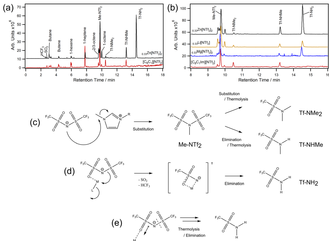
Fig. 4 TD-GC-MS chromatograms for (a) [C 8 C 1 Im][NTf 2 ] (red) and [C 8 C 1 Im][NTf 2 ] 0.33 Zn[NTf 2 ] 2 (black) with peak assignments for 0–18 min; (b) chromatogram expansions from 8–16 min with [C 8 C 1 Im][NTf 2 ] 0.33 Li[NTf 2 ] 2 and [C 8 C 1 Im][NTf 2 ] 0.33 Mg[NTf 2 ] 2 for comparison; (c) decomposition scheme showing substitution and elimination routes in the absence of metals (a full scheme is shown in ESI, Scheme S1†); (d) metal–ligand interaction leading to formation of a transition state and subsequent elimination reactions; (e) simplified representation for polarisation of [NTf 2 ] - and the increased susceptibility to thermolysis.
