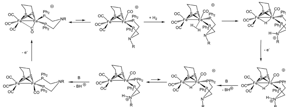
Scheme 5. Simplified version of the \text{H}_2 oxidation mechanism ( \text{R} = \text{Pr} ) proposed by Ahlquist and co-workers [13–15].
