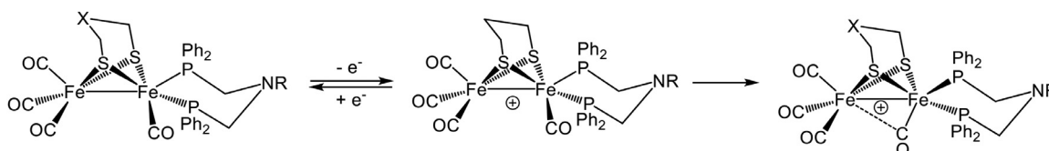
Scheme 2. Oxidation of [Fe_2(CO)_4(\mu\text{-dithiolate})\{\kappa^2\text{-(Ph}_2\text{PCH}_2)_2\text{N(R)}\}] to afford kinetically favoured all terminal CO cation which isomerises to thermodynamically favoured semi-bridging carbonyl.
