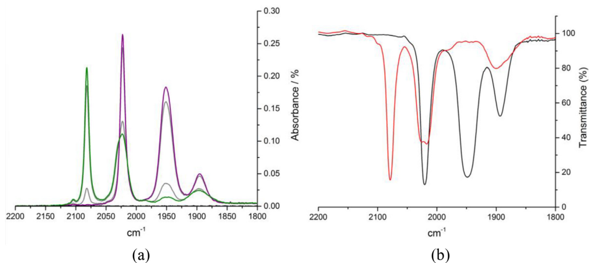
Fig. 4. (a) IR SEC of a 1 mM solution of 3 in 0.1 M TBAFP/ \text{CH}_2\text{Cl}_2 (purple = 3 , green = 3 + ); (b) chemical oxidation of 4 in \text{CH}_2\text{Cl}_2 (black = 4 , red = 4 + ). In (a) grey lines represent scans at intermediate points where multiple species exist in the solution.
