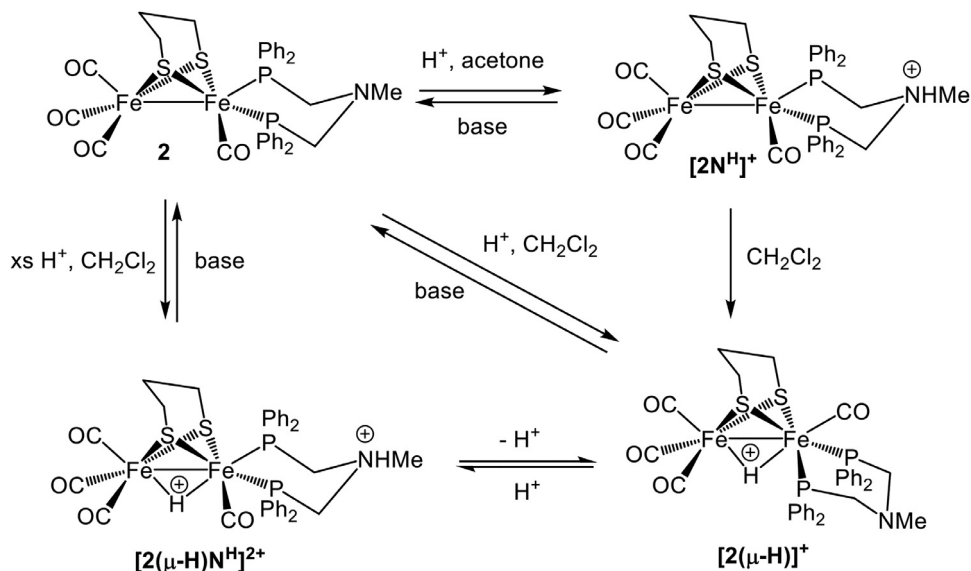
Scheme 3. Protonation chemistry of 2 with \text{HBF}_4\cdot\text{Et}_2\text{O} in \text{CH}_2\text{Cl}_2 and acetone [8].
