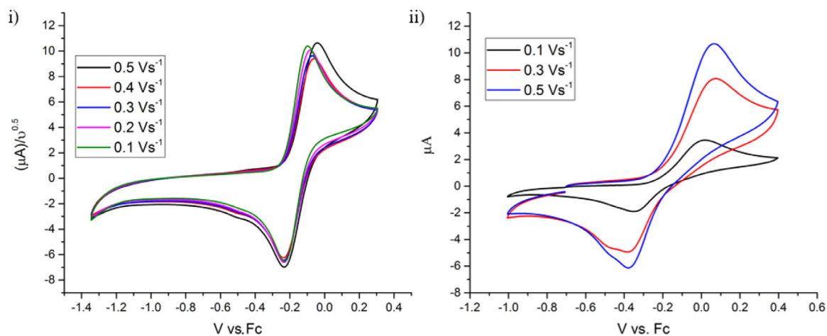
Fig. 3. CVs (1 mM solution in 0.1 M TBAFP/ \text{CH}_2\text{Cl}_2 ) of (i) 3 (normalised for scan rate), and (ii) 4 at varying scan rates.
