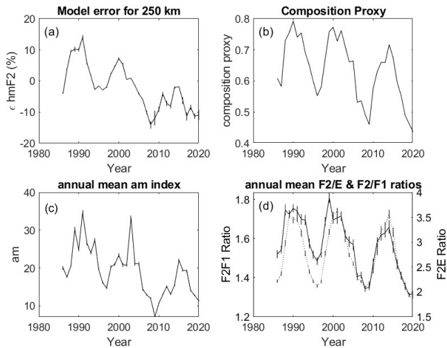
Figure 12. (a) Percentage error in the empirical hmF2 model, \epsilon_{hmF2} , after calibration with ISR data for each year in the time range 1986–2020. (b) Qualitative composition proxy based on annual average noon foF2 value scaled by solar f10.7\text{cm} flux. (c) Annual average values of the am index for the same epoch. (d) The annual average ratios in foF2/foF1 (solid line) and foF2/foE (dotted line) for the same epoch.
