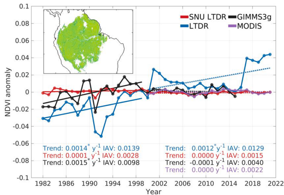
Fig. A9. Annual growing season anomaly of four NDVI datasets in Amazon evergreen broadleaf forests (AVHRR LTDR , AVHRR harmonized , GIMMS3g, and MODIS). Slope and interannual variability were calculated in different periods (Upper left: 1982–1999; Below right: 2000–2021; GIMMS3g: 2000–2015). The different colors represent AVHRR LTDR (LTDR) (blue), AVHRR harmonized (SNU LTDR) (orange), GIMMS3g (green), and MODIS (purple) NDVI, respectively. (For interpretation of the references to colour in this figure legend, the reader is referred to the web version of this article.)
