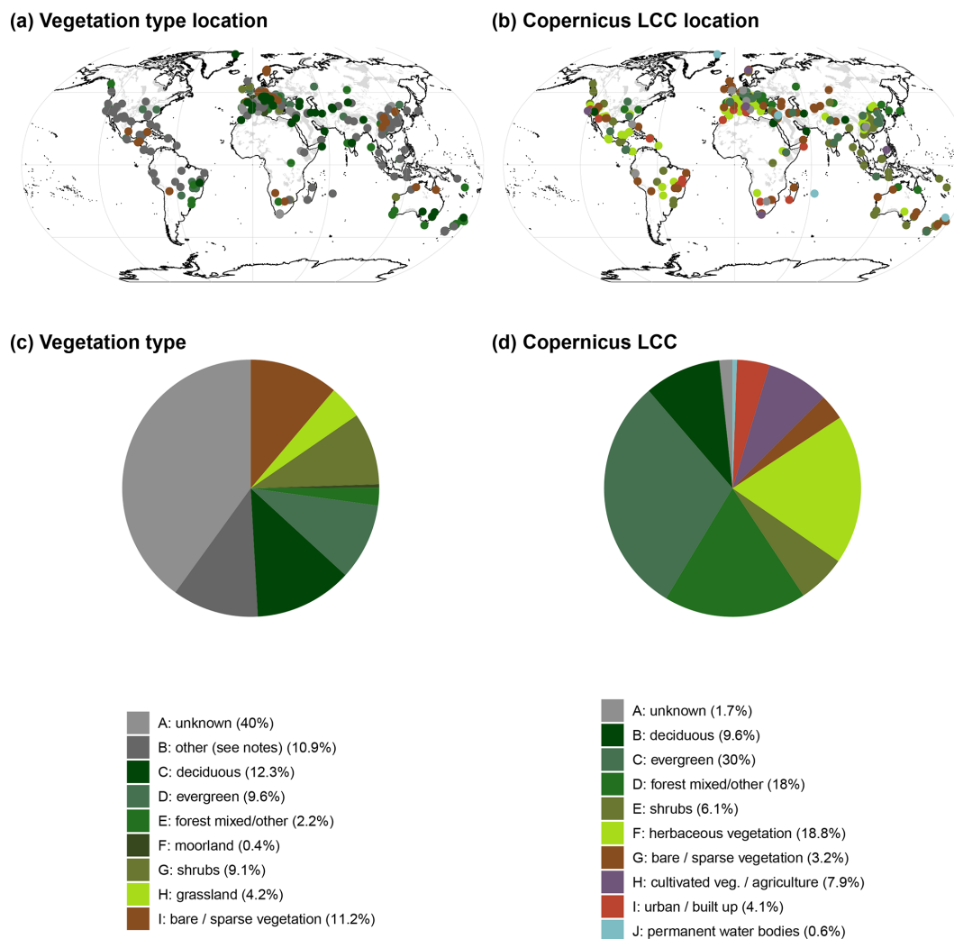
Figure 9. (a) Vegetation description from the original publications or provided by authors and (b) land cover categories extracted from the Copernicus LCC database (Buchhorn et al., 2021, 2020) with a radius of 250 m around the cave sites. (c) Pie chart showing the relative proportions of vegetation types as reported by authors. (d) Pie chart showing the relative proportions of land cover types as extracted from the Copernicus LCC database. Background shading in the map shows the global karst distribution extracted from the World Karst Aquifer Map (WoKAM; Goldscheider et al., 2020). To allow comparison between the two datasets, the Copernicus LCC vegetation data were grouped into broader categories, e.g. “deciduous” includes all closed and open broadleaf and needleleaf forest marked as deciduous. The entries in the database are more detailed.
