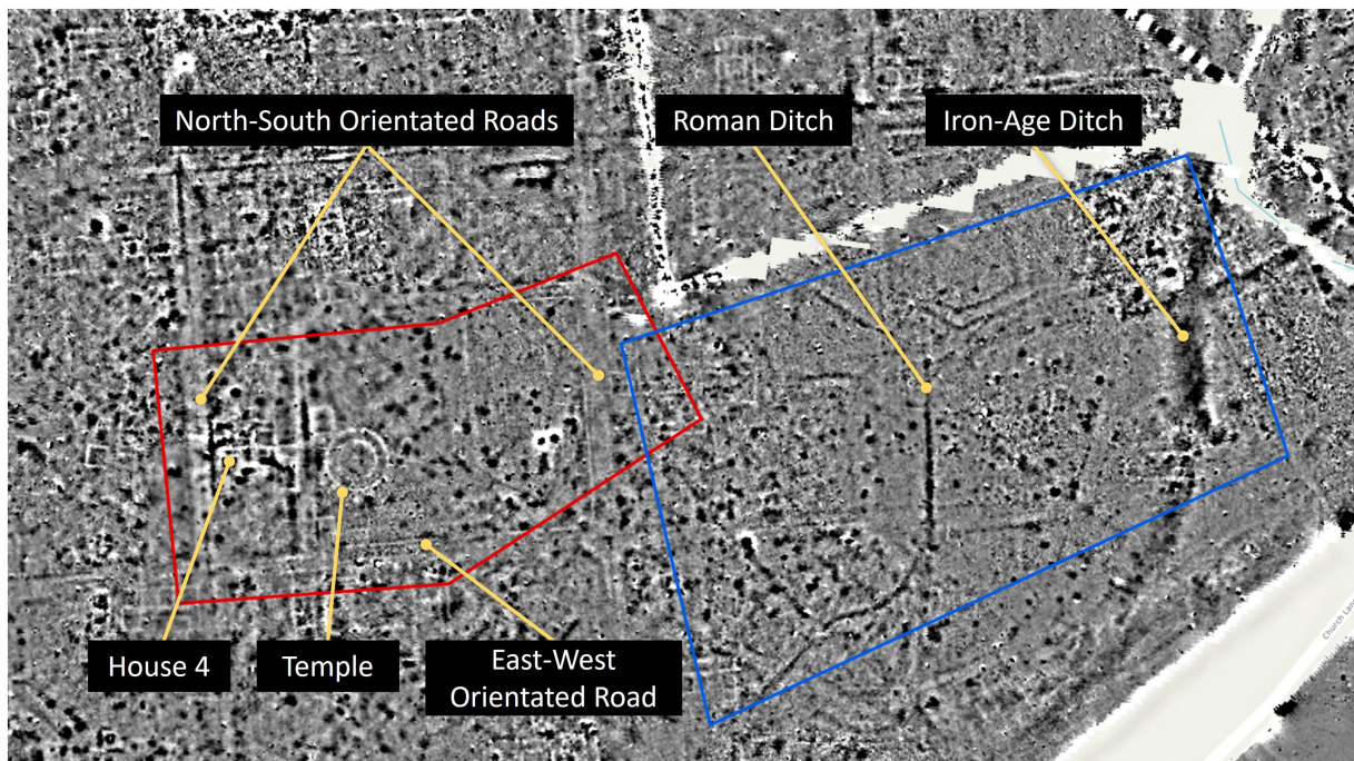
FIGURE 2 | Close-up view of the survey areas overlaying the fluxgate gradiometer data ( \pm 7\text{nT} —black high to white low). The figure shows the targets present within Area A (outlined in red) and Area B (outlined in blue).
