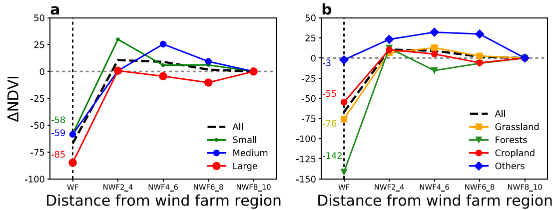
Figure 6. Influences of wind farm size (a), land cover (b), and distance to wind farms on \Delta\text{NDVI} . (a) \Delta\text{NDVI} is shown as a function of wind farm size and distance to wind farms. (b) \Delta\text{NDVI} is shown as a function of land cover types and distance to wind farms. \Delta\text{NDVI} of WF is calculated as the peak NDVI difference between WF and reference NWF areas NWF8_10 following equation (2). \Delta\text{NDVI} of NWF2_4 is calculated as the peak NDVI differences between NWF2_4 and NWF8_10, and the same for \Delta\text{NDVI} of NWF4_6 and NWF6_8. The vertical dotted line highlights the WF area. Note that the displayed NDVI values are multiplied by 10 000.
