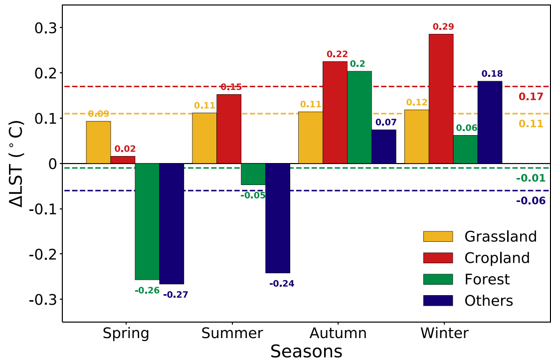
Figure 7. Influences of land cover type on nighttime \Delta\text{LST} . Seasonal \Delta\text{LST} is shown in the bar chart as a function of land cover types (grassland, forests, cropland, and others). The annual mean \Delta\text{LST} of different land cover types is shown by horizontal dashed lines.
