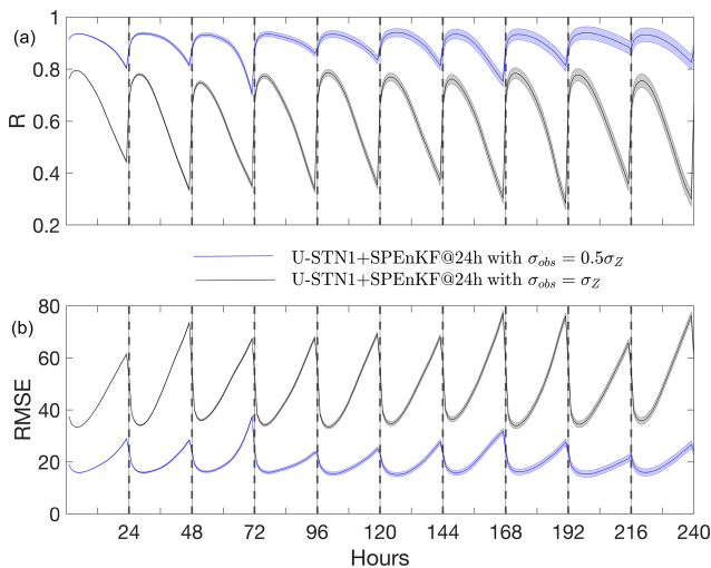
Figure 5. Panel (a) shows R and panel (b) shows RMSE (in meters) between noise-free data from ERA5 and the forecasts from U-STN1+SPEnKF for two levels of observation noise. Predictions are started from 30 random noisy observations. The lines (shading) show the mean (standard deviation) of the 30 forecasts. Noisy observations are assimilated every 24 h (indicated by black, dashed vertical lines).
