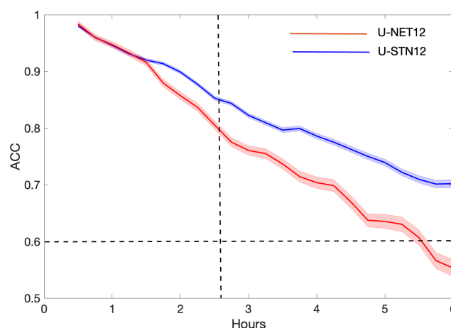
Figure A1. Performance of U-STN12 and U-NET12 on T850. Shading represents standard deviation over 30 initial conditions.
