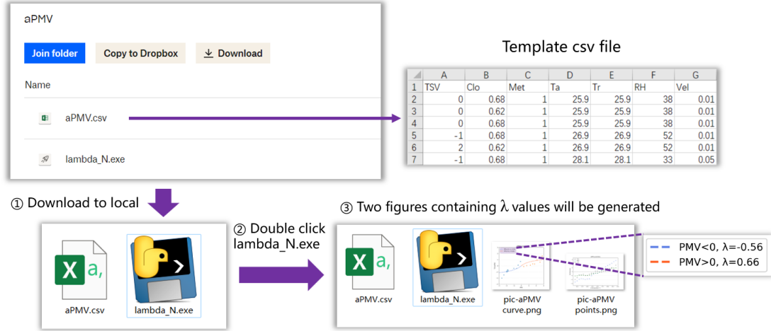
Fig. 11 Steps of using executable EXE file for solving \lambda_N without Python installation
