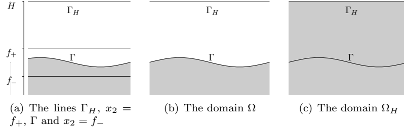
Figure 1: The domain for the boundary value problem
