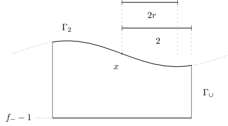
Figure 2: The point x , the surfaces \Gamma_2 and \Gamma_\cup .
