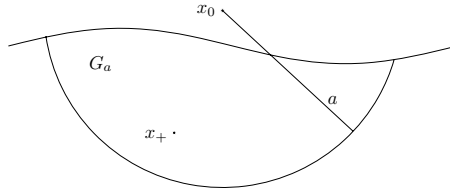
Figure 5: The domain G_a and points x_0, x_+ .
