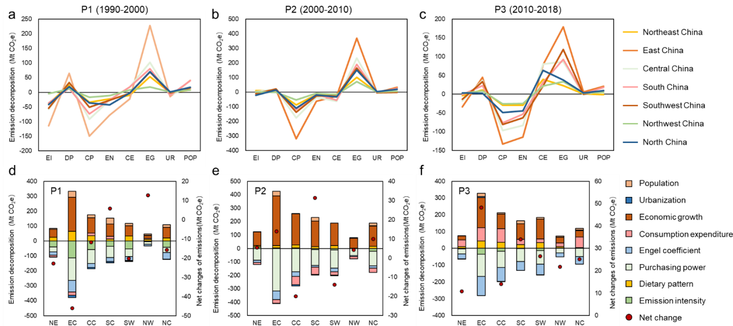
Figure 5 Change rate and decomposition of food system GHGs from seven regions in China. EI represents effects of technology, DP represents effects of dietary pattern, CP represents effects of purchasing power, EN represents effects of Engel coefficient, CE represents effects of consumption expenditure, EG represents effects of economic growth, UR represents effects of urbanization, POP represents effects of population. Parts a, b, c respectively represent the comparison of regional drivers in three periods. Parts d, e, f represent the decomposition results of regions in these periods respectively. P1 represents the period of 1990-2000, P2 represents the period of 2000-2010, and P3 represents the period of 2010-2018.
