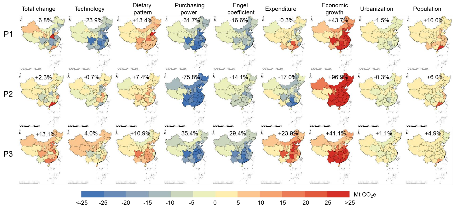
Figure 6 Spatial patterns in total food system GHGs emissions changes in China and the role of eight drivers between 1990 and 2018. Percentage values indicate the contribution made by each driver to overall. P1, P2 and P3 represent the periods of 1990-2000, 2000-2010, and 2010-2018, respectively.
