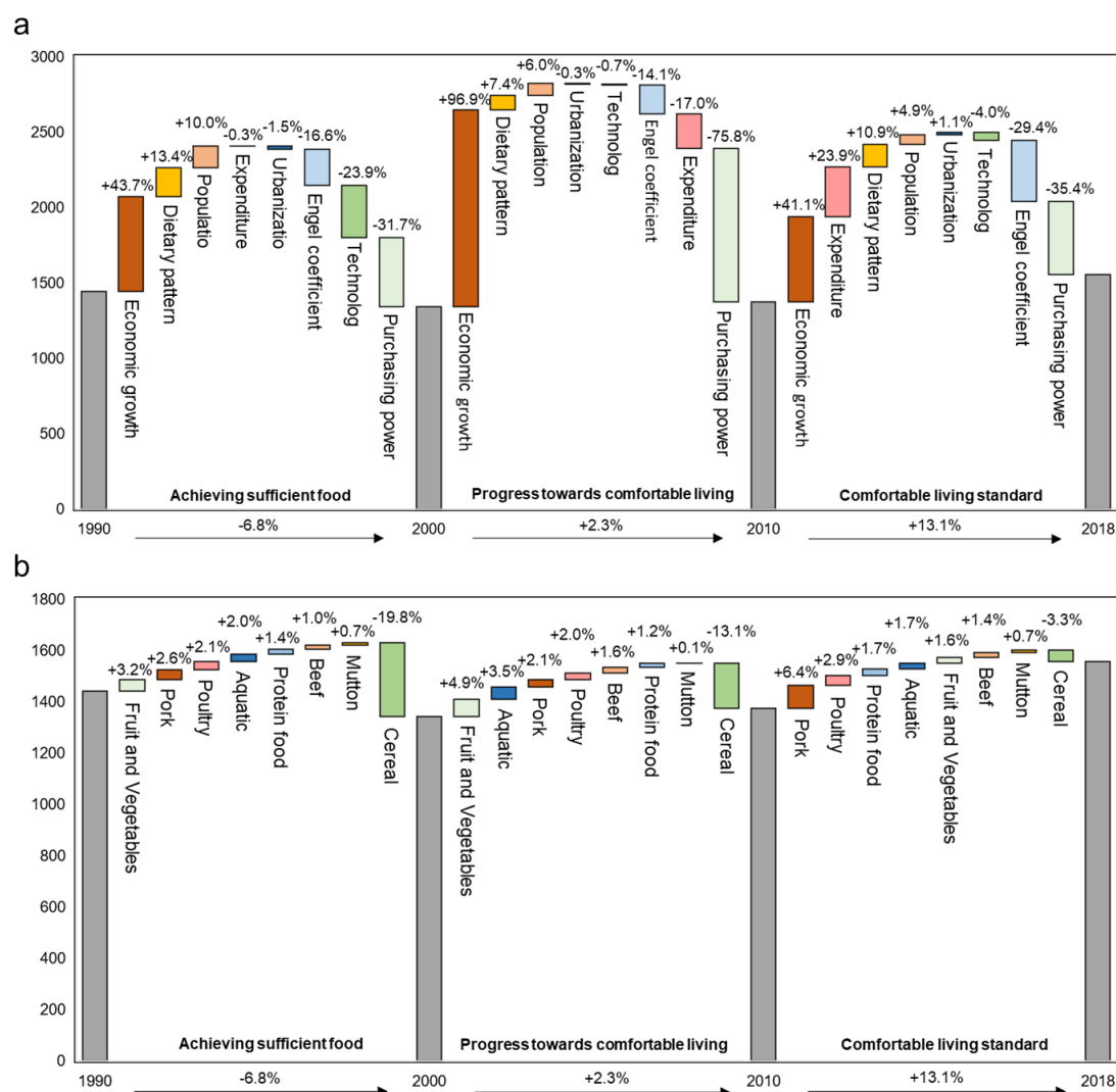
Figure 4. Contribution to the changes of GHGs from China's food system in three periods. a. Contribution of different factors of GHGs in food system in three periods. b. Contribution of different food types of GHGs in food system in three periods. According to the classification standard of the Engel coefficient used by the FAO these periods are 1990–2000 (P1) - achieve sufficient food, Engel's range 50%–59%; 2000–2010 (P2) – progress towards comfortable
