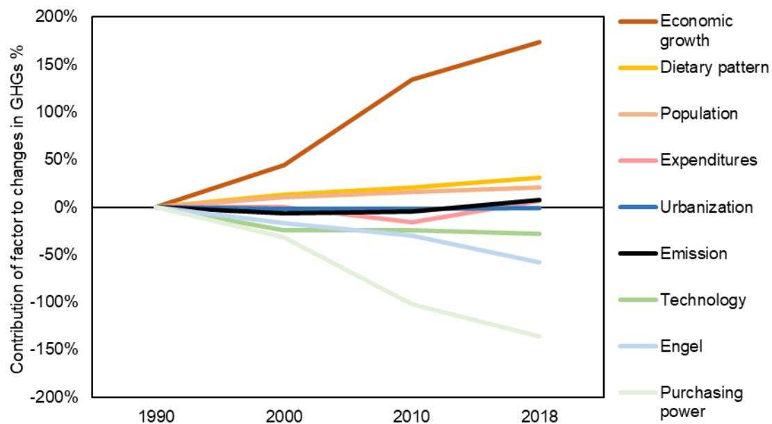
Figure 3. Contributions of different factors to changes in food system GHGs between 1990 and 2018. Using 1990 as the base year, the solid black line shows the percentage change in total food system GHGs. The other lines show the contribution to the change in emissions from eight different drivers.
