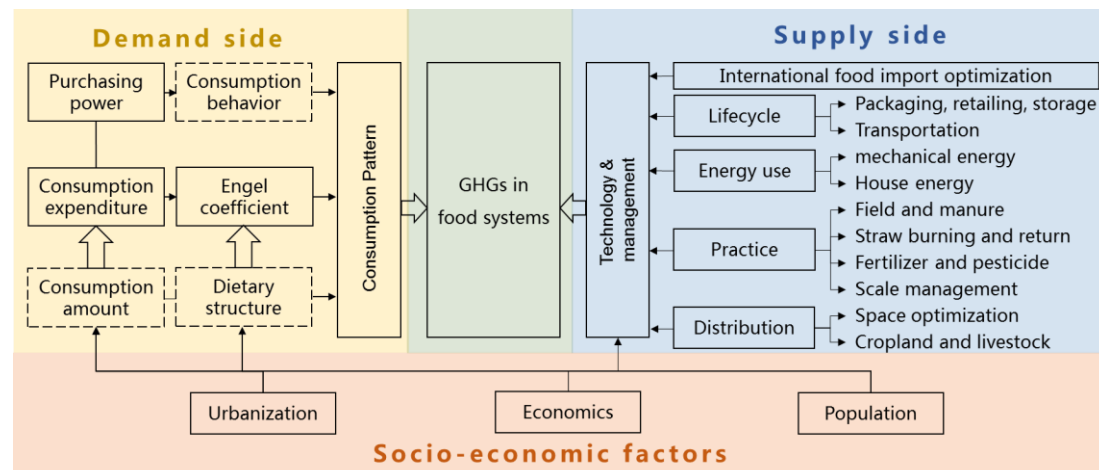
Figure 1. Framework of mechanisms influencing GHGs emissions from the food system in China.
