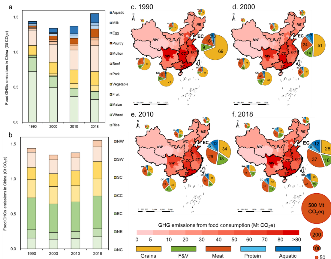
Figure 2. Spatial-temporal changes of China's food system emissions. a. China's total food system emissions related to food types; b. China's total food system emissions related to regions; c-f. represent the spatial distribution of food system emissions in China from 1990 to 2018. Different shades of red on the maps represent changes in total GHGs from regional food systems. Colors in the pie charts represent different food types with numbers representing percentages of the total. The sizes of pie charts correspond to emission amounts. Grains comprise rice, wheat, and maize; F&V comprise fruit and vegetables; meat comprises pork, beef, mutton, and poultry; protein comprises eggs and milk; and aquatic comprises fish, shrimp, crab, shellfish, and algae
