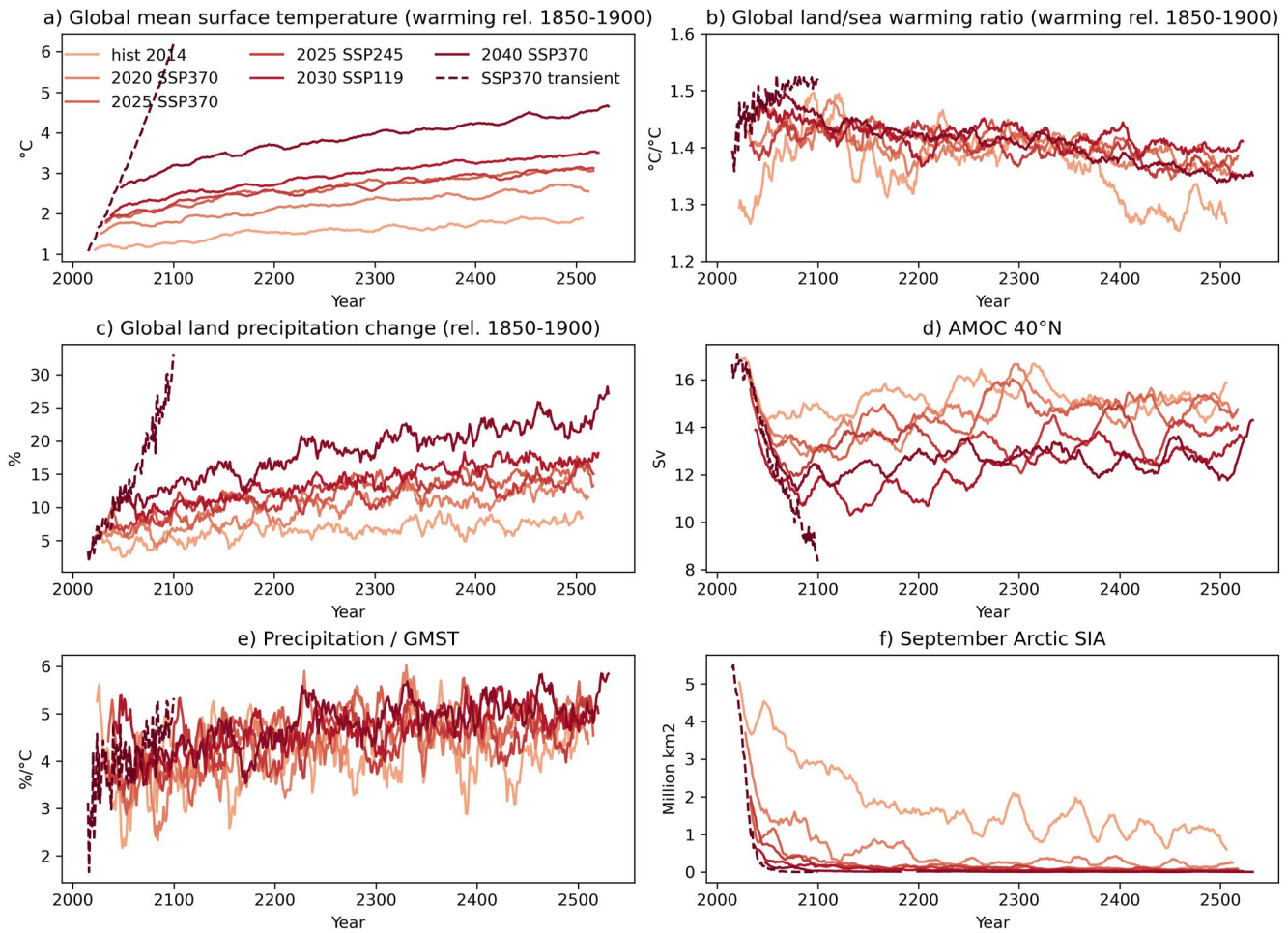
Figure 1. 16-year running means of global mean surface air temperature (GSAT) (a), the land-sea warming ratio (b), global land precipitation (c), the Atlantic Meridional Overturning Circulation at 40°N (d), hydrological sensitivity defined as global land precipitation divided by GSAT (e), and September Arctic sea-ice area (f) in the various simulations. The reference time period for anomalies (panels a–c) is 1850–1900. The SSP3-7.0 transient projections are a 16-member ensemble mean and are not temporally smoothed.
