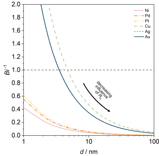
Figure 7. Dependency of the Biot number, in the form of Bi^{-1} , on the particle size, d . The curves are referred to the thermal conductivity of the liquid, \kappa_L , and the interfacial thermal resistance with each metal, R_K , at T = 298 K.
