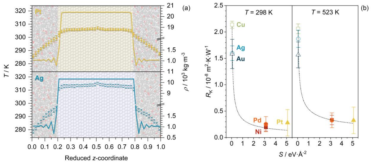
Figure 6. (a) Temperature (scatter) and density (solid line) profiles of the atomistic models of metal-molecular liquid interfaces with Pt and Ag, at average T = 298 \text{ K} . (b) Relationship between the thermal resistance (calculated at either T = 298 \text{ K} or T = 523 \text{ K} ) and the stiffness of the metal-carbon interaction at the interface.
