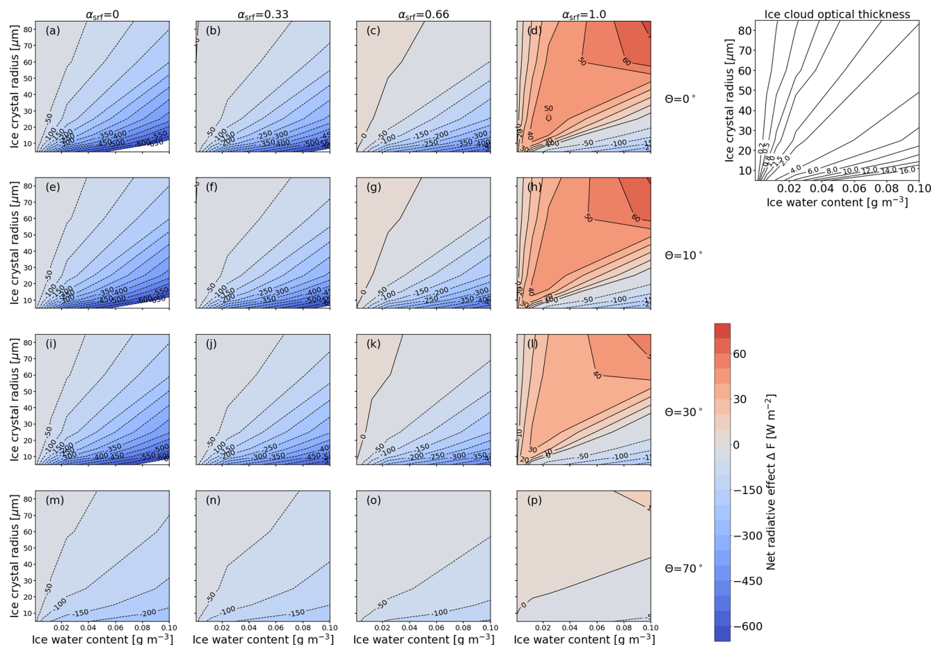
Figure 11. Same as Fig. 10 but for \Delta F_{\text{net}} (in \text{W m}^{-2} ).
