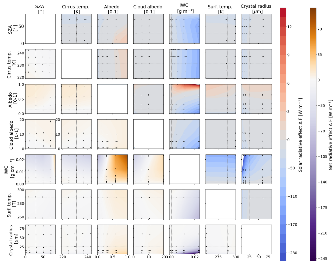
Figure A1. The upper diagonal panels show the plot of median solar \Delta F_{\text{sol}} projected in a 2D parameter space. Blue colors indicate negative \Delta F_{\text{sol}} (cooling), while red colors indicate positive \Delta F_{\text{sol}} (warming). The lower diagonal panels show the same as the upper diagonal panels but for median net \Delta F_{\text{net}} . Purple shades indicate negative \Delta F_{\text{net}} (cooling), while orange shades indicate positive \Delta F_{\text{net}} (warming). All \Delta F have the same units (given in \text{W m}^{-2} ). The black arrows point to the direction of the steepest slope.
