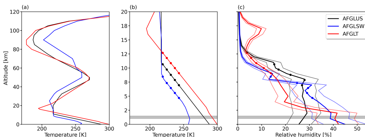
Figure B1. Profiles of temperature (a, b) and relative humidity (c) used for the radiative transfer simulations. The sub-Arctic ( afglsw ), mid-latitude ( afglus ), and tropical ( afglt ) profiles are given in blue, black, and red, respectively. The modified profiles with \pm 20 % are indicated by pale colors. The positions of the simulated ice water cloud are indicated by the colored dots for each profile. The position of the low-level liquid water cloud is indicated by the gray shaded area.
