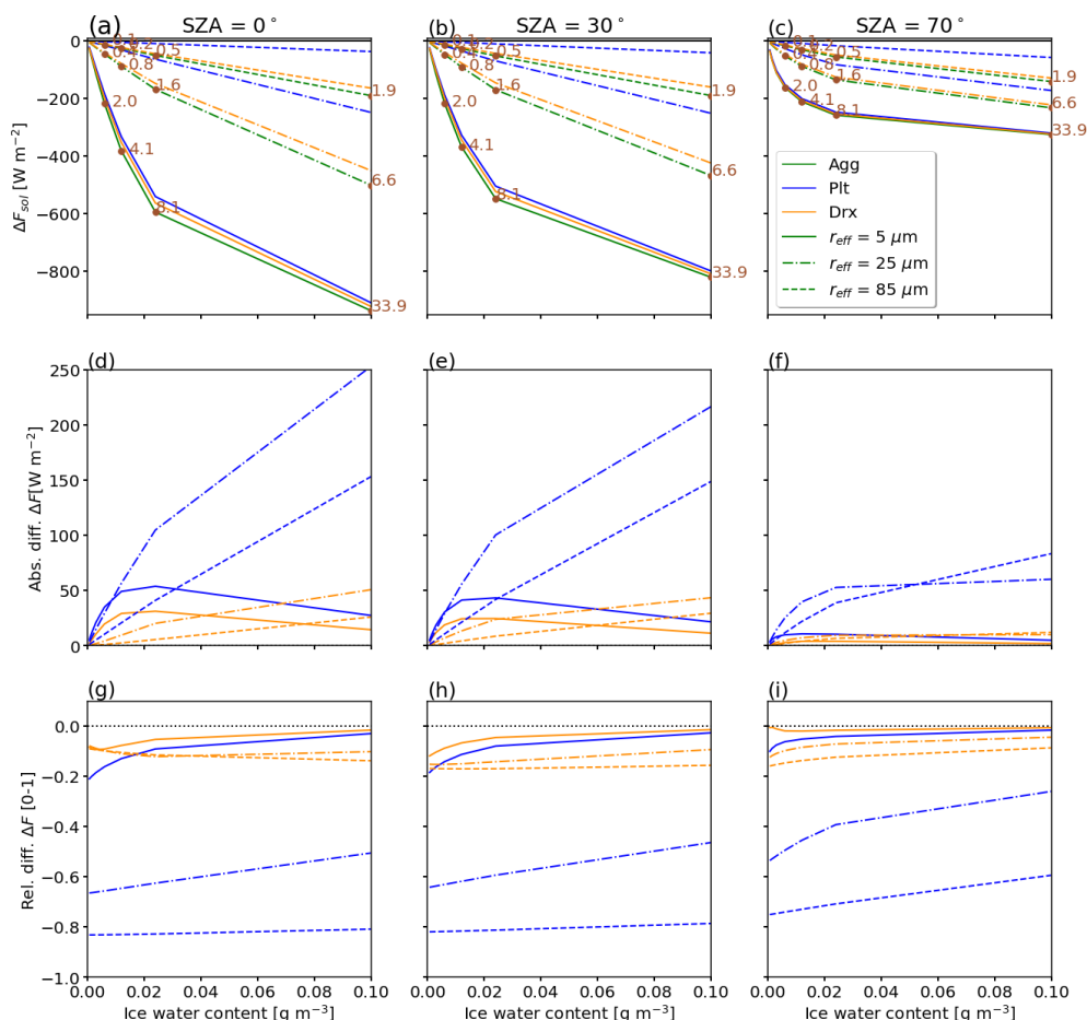
Figure 3. (a–c) Solar radiative effect \Delta F_{\text{sol}} (in W m -2 ) as a function of ice water content IWC for three values of the solar zenith angle with \theta of 0, 30, and 70°. Three ice crystal radii r_{\text{eff}} of 5 (solid), 25 (dash-dotted), and 85 \mu\text{m} (dashed) are indicated. The ice crystal shape is color coded, with the aggregates “Agg”, plates “Plt”, and droxtals “drx” given in green, blue, and orange, respectively. Panels (d)–(f) show the absolute difference and panels (g)–(i) show the relative difference between \Delta F_{\text{sol}} of droxtals and plates with respect to aggregates with the same crystal radius. The numbers indicate the optical thickness simulated for the reference that contains ice aggregates.
