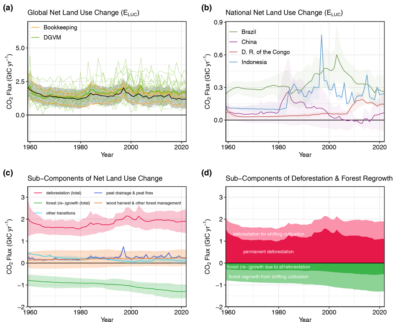
Figure 7. Net \text{CO}_2 exchanges between the atmosphere and the terrestrial biosphere related to land-use change. (a) Net \text{CO}_2 emissions from land-use change ( E_{\text{LUC}} ) with estimates from the three bookkeeping models (yellow lines) and the budget estimate (black with \pm 1\sigma uncertainty), which is the average of the three bookkeeping models. Estimates from individual DGVMs (narrow green lines) and the DGVM ensemble mean (thick green line) are also shown. (b) Net \text{CO}_2 emissions from land-use change from the four countries with the largest cumulative emissions since 1959. Values shown are the average of the three bookkeeping models, with shaded regions as \pm 1\sigma uncertainty. (c) Sub-components of E_{\text{LUC}} : (i) emissions from deforestation (including permanent deforestation and deforestation in shifting cultivation cycles), (ii) emissions from peat drainage and peat fires, (iii) removals from forest (re)growth (including forest (re)growth due to afforestation and reforestation and forest regrowth in shifting cultivation cycles), (iv) fluxes from wood harvest and other forest management (comprising slash and product decay following wood harvest, regrowth after wood harvest, and fire suppression), and (v) emissions and removals related to other land-use transitions. The sum of the five components is E_{\text{LUC}} shown in panel (a). (d) Sub-components of “deforestation (total)” and of “forest (re)growth (total)”: (i) deforestation in shifting cultivation cycles, (ii) permanent deforestation, (iii) forest (re)growth due to afforestation and/or reforestation, and (iv) forest regrowth in shifting cultivation cycles.
