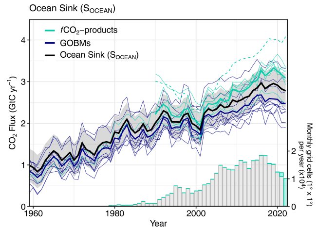
Figure 10. Comparison of the anthropogenic atmosphere–ocean \text{CO}_2 flux showing the budget values of S_{\text{OCEAN}} (black, with the uncertainty in grey shading), individual ocean models (royal blue), and the ocean f\text{CO}_2 products (cyan, with Watson et al., 2020, represented by a dashed line as not used for ensemble mean). Only one f\text{CO}_2 product (Jena-MLS) extends back to 1959 (Rödenbeck et al., 2022). The f\text{CO}_2 products were adjusted for the pre-industrial ocean source of \text{CO}_2 from river input to the ocean by subtracting a source of 0.65 \text{ Gt C yr}^{-1} to make them comparable to S_{\text{OCEAN}} (see Sect. 2.5). The bar plot on the lower right illustrates the number of f\text{CO}_2 observations in the SOCATv2023 database (Bakker et al., 2023). Grey bars indicate the number of data points in SOCATv2022 and coloured bars the newly added observations in v2023.
