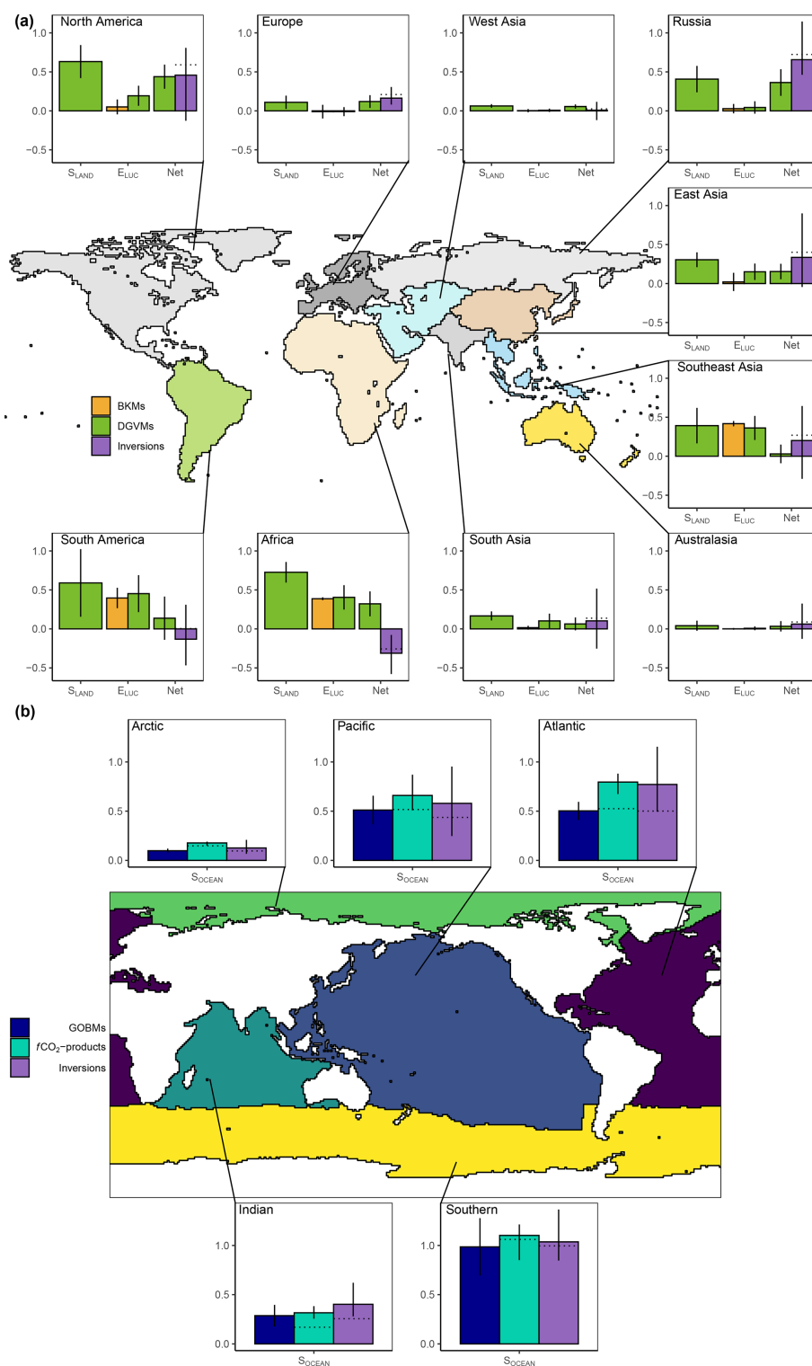
Figure 14. Decadal mean (a) land and (b) ocean fluxes for RECCAP-2 regions over 2013–2022. For land fluxes, S_{\text{LAND}} is estimated by the DGVMs (green bars), with the error bar as \pm 1\sigma spread among models. A positive S_{\text{LAND}} value is a net transfer of carbon from the atmosphere to the land. E_{\text{LUC}} fluxes are shown for both DGVMs (green) and bookkeeping models (BKM; orange), again with the uncertainty calculated as the \pm 1\sigma spread. Note that a positive E_{\text{LUC}} flux indicates a loss of carbon from the land. The net land flux is shown for both DGVMs (green) and atmospheric inversions (purple), including the full model spread for inversions. The net ocean sink ( S_{\text{OCEAN}} ) is estimated by GOBMs (royal blue), f\text{CO}_2 products (cyan), and atmospheric inversions (purple). Uncertainty is estimated as the \pm 1\sigma spread for GOBMs and the full model spread for the other two products. The dotted lines show the f\text{CO}_2 products and inversion results without river flux adjustment. Positive values are \text{CO}_2 sinks.
