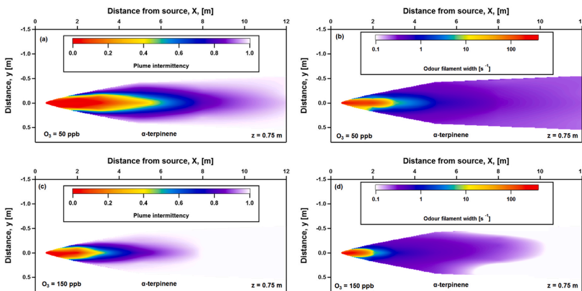
Fig. 6. Panels a and c, show the intermitty of an \alpha -terpinene plume, defined as the fraction of time (0–1) that the measured signal fell below the threshold of perception (see text for definition), under identical turbulent conditions but varying ozone concentrations of 50 ppb and 150 ppb, respectively. Panels b and d show the average odour filament width from the same \alpha -terpinene plumes. Note the colour scale in panels b and d are shown on a logarithmic scale.
