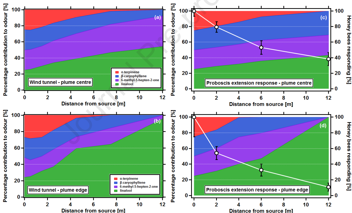
Figure 7 Observed ratios of α-terpinene, β-caryophyllene, 6-methyl-5-hepten-2-one (MHO) and linalool measured at the plume centre (panel a) and plume edge (panel b) under an ozone field of 150 ppb. Panels c and d show an attempt to replicate these ratios as part of a proboscis extension response assay, for the plume centre and plume edge, respectively. The right hand axis and line graphs on panels c and d indicate the percentage of forager honeybees which, after learning the four VOC blend representative of 0 m from the source, extended their proboscis (indicating recognition) when presented with VOC blends representative of 2, 6 and 12 m from the source ( \pm S.E.). Data are expressed as the percent PER recognition of each distance relative to the PER recognition of blend at the source ( n = 34 and 37 individuals for the plume centre and plume edge, respectively). While there was no significant two-way interactive effect of 'distance from the source' and 'location of the plume', both were individually significant. As such, significantly fewer honeybees responded to the VOC blend corresponding to the
