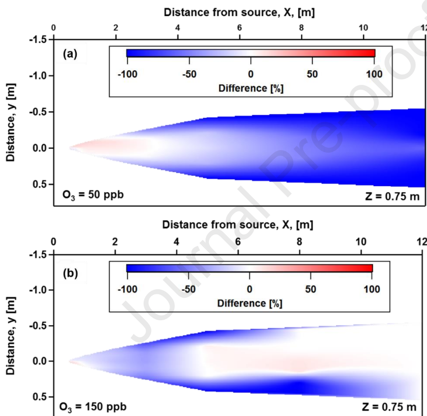
Figure 3 shows the percentage difference between an a-terpinene plume predicted based on literature rate constants and that measured by the PTR-QiTOF (e.g. measured – predicted)/predicted). Panel a and b show the difference plot under ozone conditions of 50 ppb and 150 ppb of ozone, respectively. Both plumes were released from a height of 0.75 m.
