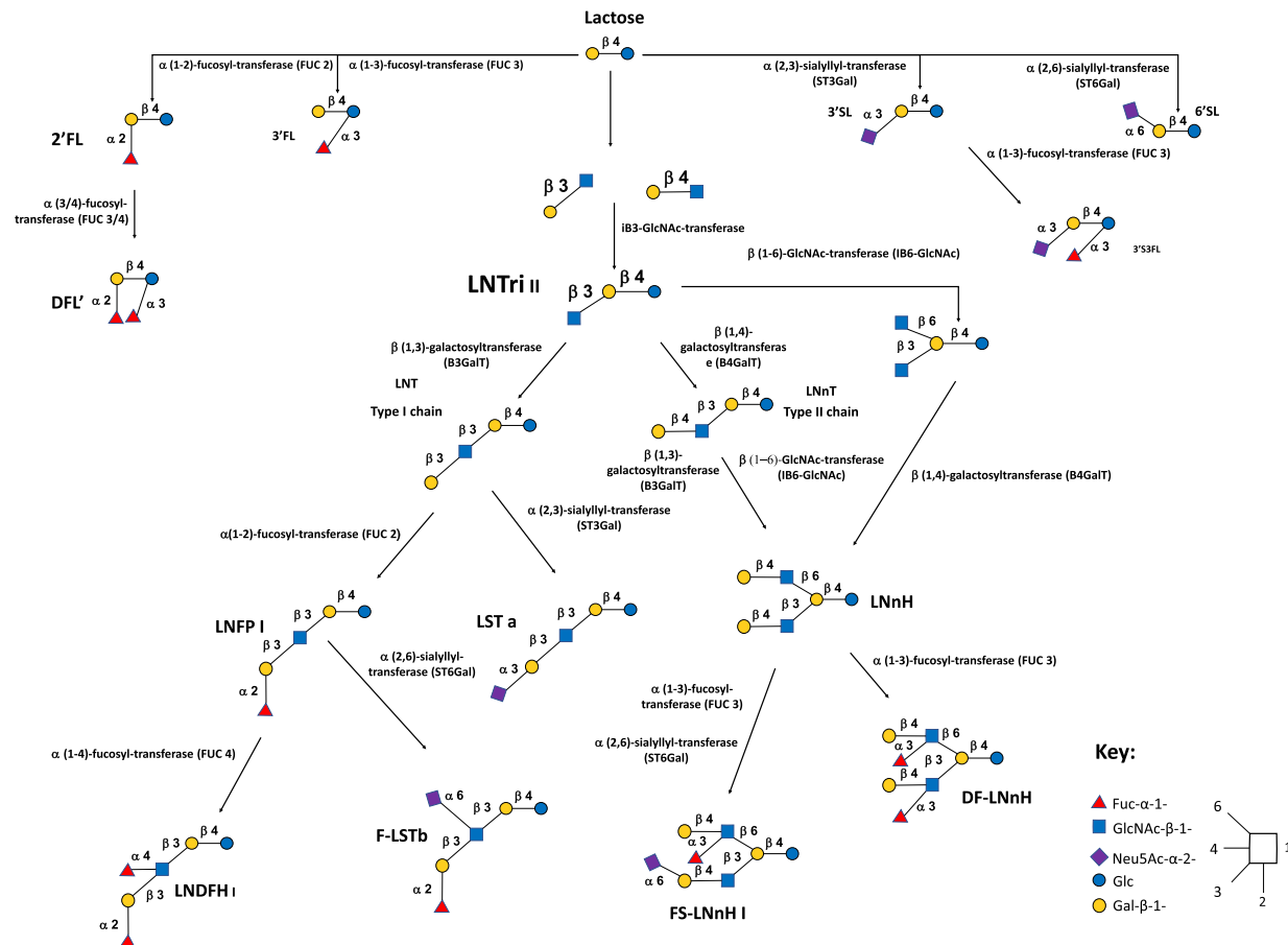
Figure 1. Generalised overview of the complexity and structural diversity of human milk oligosaccharides (HMOs) present in breast milk. Abbreviations: Neutral HMOs: 2'FL, 2'-fucosyllactose; 3'FL, 3'-fucosyllactose; DFL, difucosyllactose; DF-LNnH, difucosylated lacto-N-neohexaose; LNDFH I, lacto-N-difucohexaitol I; LNFP I, lacto-N-fucopentaose I; LNnH, lacto-N-neohexaose; LNnT, lacto-N-neotetraose; LNT, lacto-N-tetraose. Acidic non-fucosylated HMOs : 3'SL, 3'-sialyllactose; 6'SL, 6'-sialyllactose; LST a, sialyllacto-N-tetraose a. Acidic fucosylated HMOs : 3'S3FL, 3'-Sialyl-3-fucosyllactose; F-LST b, sialylfucosyllacto-N-tetraose b; FS-LNH I, fucosylsiallacto-N-hexose I.
