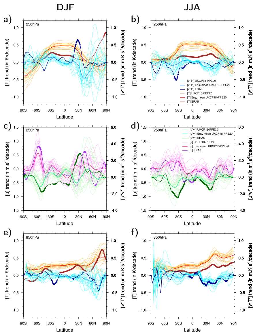
Fig. 4 Trends in poleward eddy heat and momentum fluxes (1979–2019), given by [v^*T^*] and [u^*v^*] , where the brackets denote a zonal mean and the star a deviation from that. Heavy lines denote ERA5 trends, with 5% significance indicated by dots, and thin lines the trends from the UKCP-PPE20 ensemble. a, b Temperature (orange) and heat flux (blue) at 250 hPa. c, d Zonal wind (pink) and momentum fluxes (green) at 250 hPa. e, f Temperature (orange) and heat fluxes (blue) at 850 hPa. Panels (a, c and e) are for DJF; (b, d and f) are for JJA.
