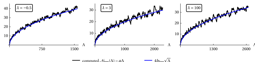
Fig. 4 The free boundary problem for the unit square. The second Weyl terms are compared to the actual numerically computed counting functions. In all three images, we take \mu = 1
