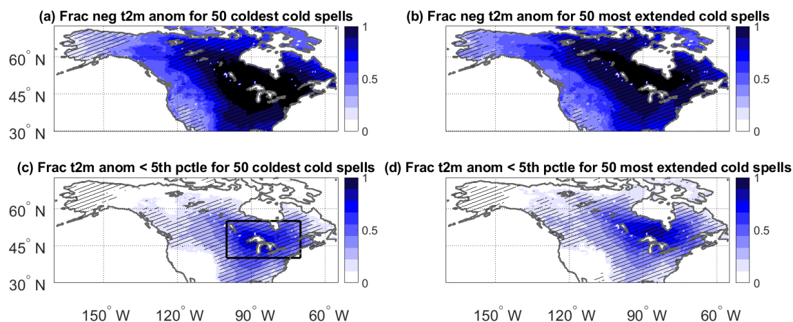
Figure A6. Fraction of negative t2m anomalies ( a, b ) and fraction of t2m anomalies below the local 5th percentile of temperature anomalies ( c, d ) for the 50 cold spells with the lowest area-averaged temperature anomaly over 40–55° N and 260–290° E ( a, c ; domain shown by the black box) and for the 50 cold spells with the most grid points below the local 5th percentile of temperature anomalies over the same domain ( b, d ). In all cases, a minimum separation of 5 d is enforced between different cold spells. Hatching denotes statistically significant anomalies, assessed as described in Sect. 2.
