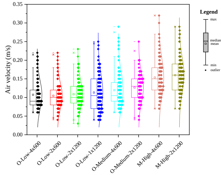
Fig. 6: The distribution of air velocity in the occupied zone with different chilled beam types.
