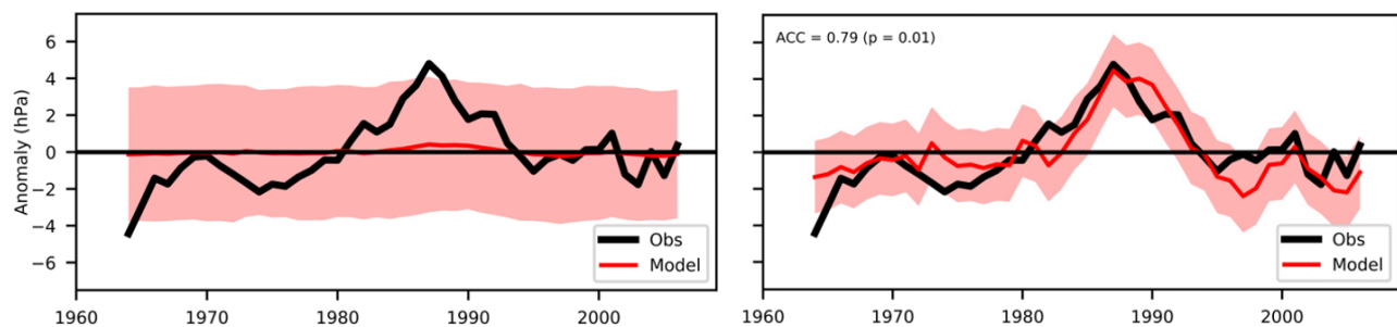
Figure 2: Decadal predictions of the NAO. Left panel: observed (black) and model-forecast (years 2–9; red) 8-yr running mean boreal winter NAO index (hPa). The red curve shows the ensemble mean; the red shading shows the 5%–95% confidence interval diagnosed from the individual members. Right panel: same as the left panel but the ensemble mean has been adjusted to have the same variance as the observations and the confidence interval has been diagnosed from the errors. Adapted from Smith et al., 2020.
