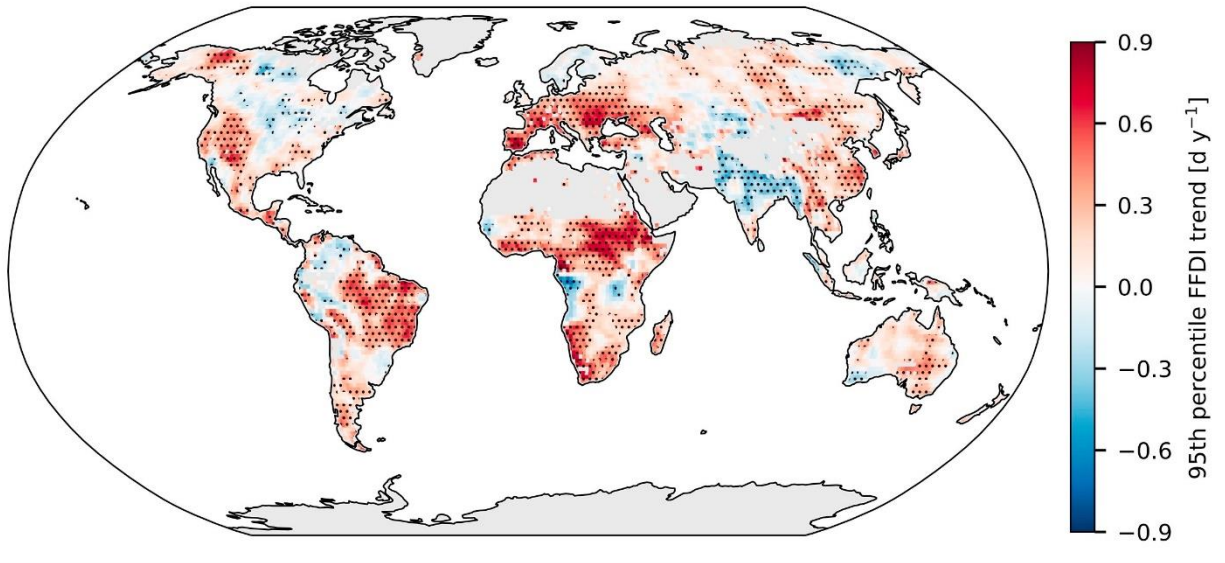
Figure 3: Trend in the number of days per year between 1970 and 2020 for which the Forest Fire Danger Index (FFDI) exceeds the climatological 95th percentile, adapted from Richardson et al. (2022). Based on data from the reanalysis product JRA55 (Japan Meteorological Agency, 2013). Shading is the Theil-Sen slope. Stippling indicates a statistically significant result from the Mann-Kendall trend test, treated for multiple testing and autocorrelation. See Richardson et al. (2022) for details.
