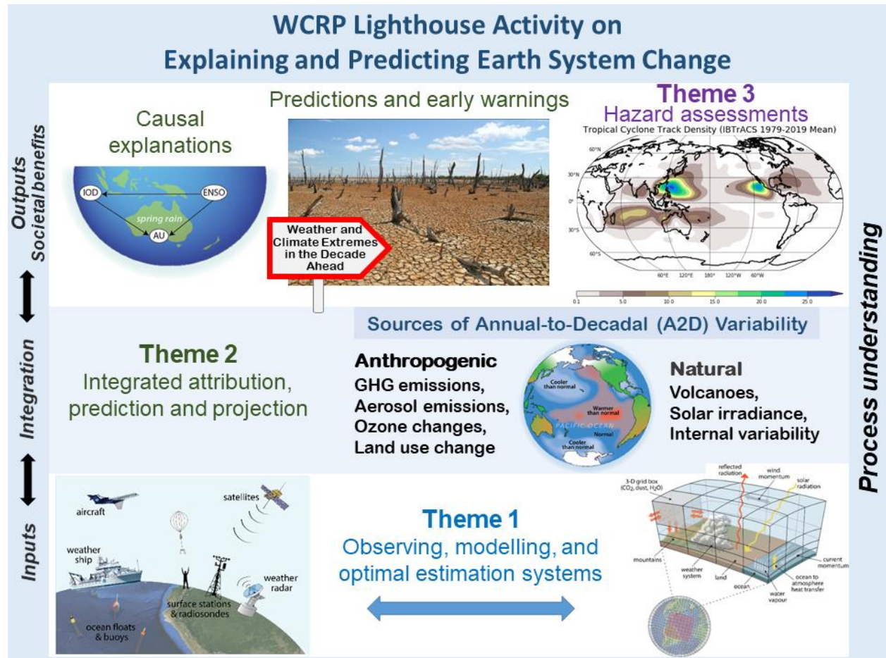
Figure 1: Key elements of the Lighthouse Activity. The bottom layer shows the importance of coordinated observational and modeling efforts serving as key tools and inputs to the integrated attribution, prediction and projection efforts in the middle layer. Both of these layers feed into the outputs and societal benefits displayed in the top layer: causal explanations, predictions and early warnings, and hazard assessments. Arrows along the left side indicate that outputs (Themes 2 and 3) and integration (Theme 2) can feedback to improve the inputs (Theme 1). Fundamental physical process understanding runs through all aspects of the Lighthouse Activity. (Causal explanations figure following Kretschmer et al., 2021.)
