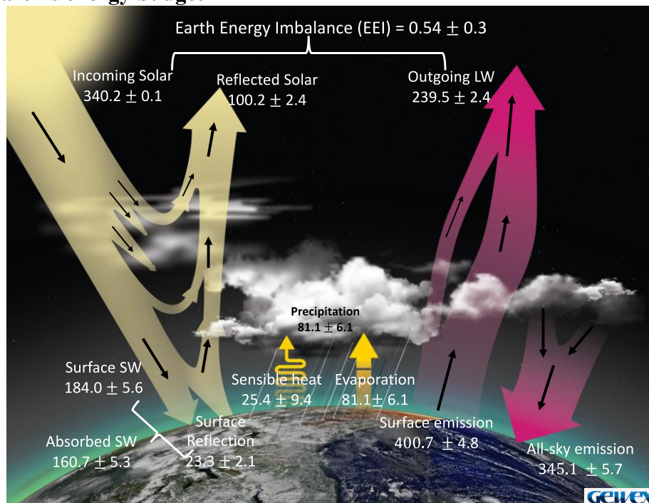
Figure SB3: An update on the mean annual fluxes of the global energy budget (all in Wm -2 ) for the first decade of the millennium. This budget was achieved using a ‘global’ optimization described in L’Ecuyer et al (2015) that requires quantitative uncertainties but uses data that produce more consistent set of fluxes.
