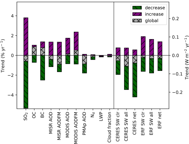
Figure 6. Mean values derived from the maps in Figs. 1 to 4, averaged over (green/downward hatching) the regions with substantial negative trends (defined as larger than 0.05 \text{ W m}^{-2} \text{ yr}^{-1} in absolute terms; isolines in Fig. 4) in ERF solar clear-sky situations from RFMIP (Fig. 4d) and (purple/upward hatching) substantial positive trends. The grey bar (crosses) is the global mean between 60^\circ \text{ S} and 60^\circ \text{ N} . The regions with negative trends cover 7.3 % of the Earth surface, the ones with positive trends, 1.1 %. The AODFM is only retrieved over oceans, and the PMap time series only spans 10 years from 2008 to 2017. From left to right: Trends in emissions of \text{SO}_2 , OC, and BC, in AOD and AODFM from MISR, MODIS, and Metop-A, in cloud droplet concentration N_d , LWP and cloud fraction from MODIS. All these are provided in units of \% \text{ yr}^{-1} and refer to the left axis. Trends in CERES retrievals of solar clear-sky, solar all-sky, and net all-sky radiation, as well as in model-derived ERF for solar clear-sky, solar all-sky, and net all-sky radiation are shown in units of \text{W m}^{-2} \text{ yr}^{-1} (right axis) and are inverted in sign: negative trends here are for reduction in magnitude (less negative fluxes/effective forcings).
