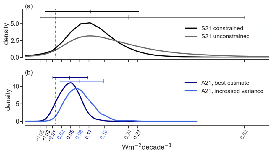
Figure 5. Assessment of the linear trend in ERFaer between 2000 and 2019. Panel (a) as in Smith et al. (2021a, their Fig. 7; abbreviated as S21 in the labels), and panel (b) as in Albright et al. (2021, labelled A21). The constraint is as in the cited studies, but applied to the period 2000–2019. Increased variance in Albright et al. (2021) corresponds to a scenario prescribing internal climate variability that is a factor of 5 larger than the CMIP6 mean and assuming large, correlated errors in global temperature observations, yielding a fifth-percentile ERFaer lower bound of -1.8 W m^{-2} . The labels along the x axis correspond to 5 % and 95 % percentiles, as well as mean, of the distribution of the curves in the corresponding colour.
