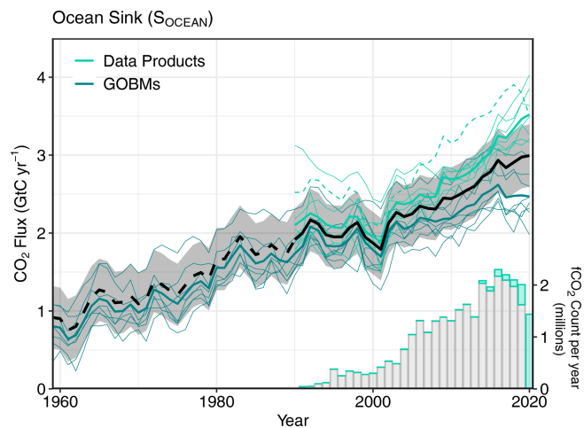
Figure 9. Comparison of the anthropogenic atmosphere–ocean \text{CO}_2 flux showing the budget values of S_{\text{OCEAN}} (black; with the uncertainty in grey shading), individual ocean models (teal), and the ocean f\text{CO}_2 -based data products (cyan; with Watson et al. (2020) in dashed line as not used for ensemble mean). The f\text{CO}_2 -based data products were adjusted for the pre-industrial ocean source of \text{CO}_2 from river input to the ocean, by subtracting a source of 0.61 \text{ GtC yr}^{-1} to make them comparable to S_{\text{OCEAN}} (see Sect. 2.4). Bar-plot in the lower right illustrates the number of f\text{CO}_2 observations in the SOCAT v2021 database (Bakker et al., 2021). Grey bars indicate the number of data points in SOCAT v2020, and coloured bars the newly added observations in v2021.
