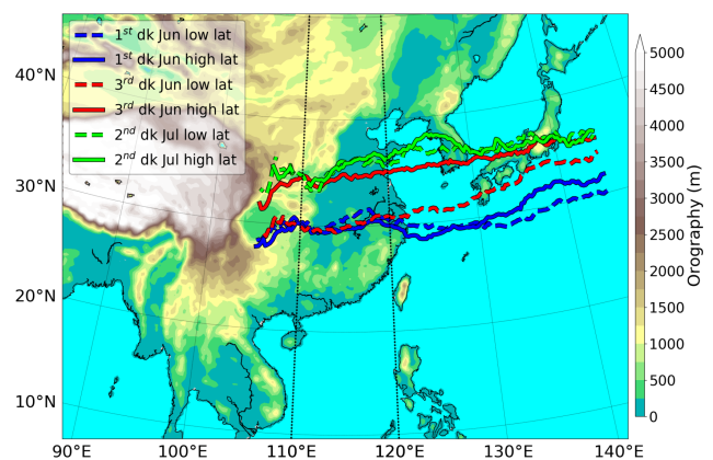
Figure 13. Dekadal mean location of EASM frontal band at 850 hPa. As in Fig. 2, but for high-lat and low-lat years and only for selected decades (see legend).
