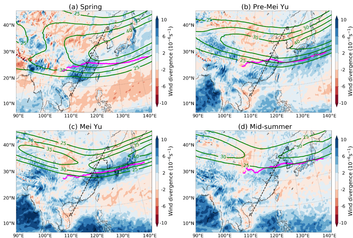
Figure 8. Dekadal mean horizontal wind divergence at 200 hPa (shading; 10^{-6} \text{ms}^{-1} ) and magnitude of horizontal wind speed at 200 hPa (green contours; every 5 \text{ms}^{-1} from 25 \text{ms}^{-1} upwards). The magenta line indicates the climatology of the mean dekadal location of the EASMF at 850 hPa. The AB dashed black line indicates the transect of the vertical cross-section in Fig. 10. The dekads representing the four stages of EASM progression (first dekad of May, first dekad of June, third dekad of June, second dekad of July, respectively) are selected according to Fig. 3. Data from ERA5 1979–2018 climatology.
