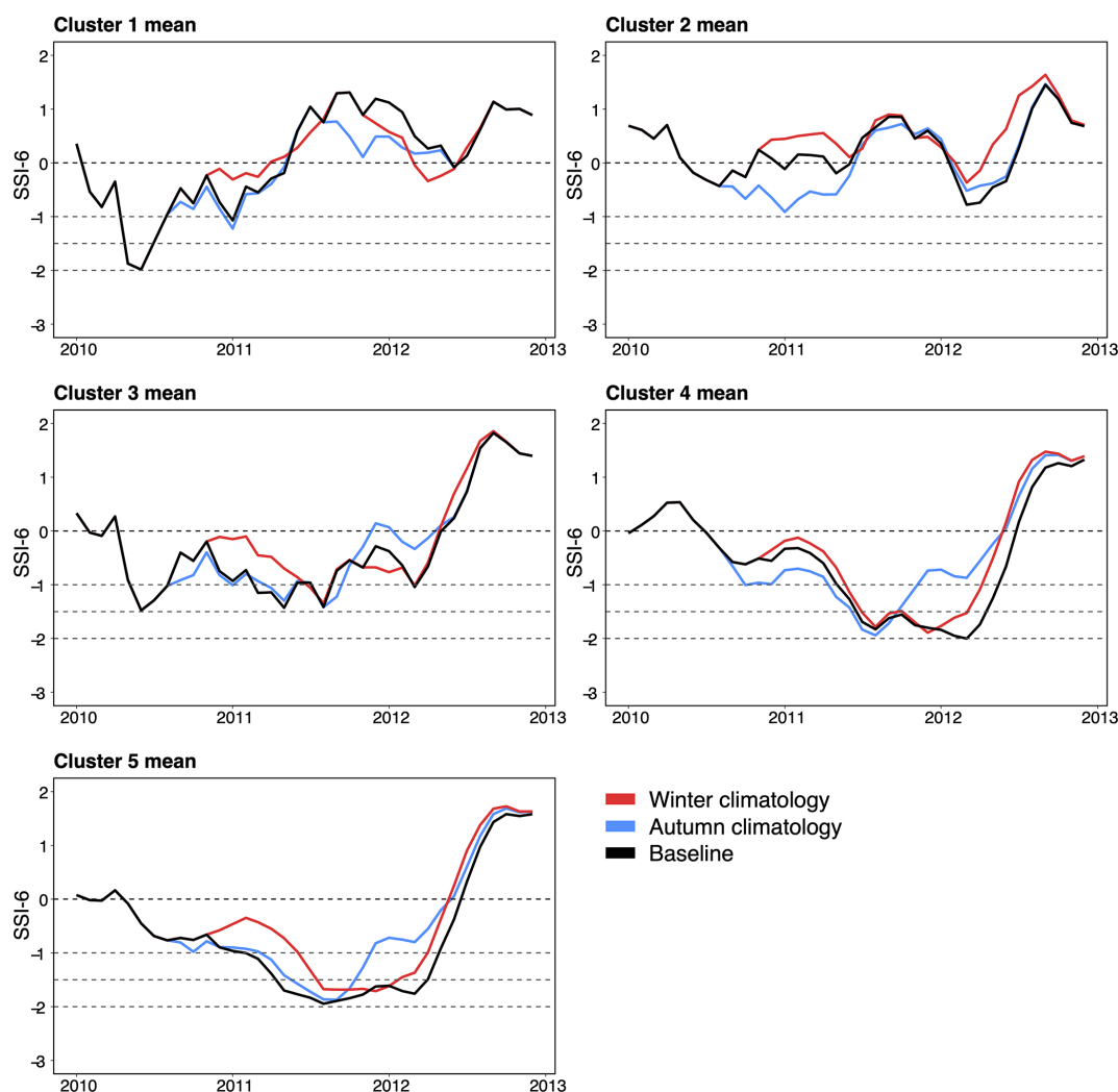
Figure 5. Cluster mean SSI-6 for the storylines of seasonal contributions with winter 2010/2011 (red) and with autumn 2010 and 2011 (blue) replaced by daily climatological values. See Figs. S5 and S6 for the equivalent figure for SSI-12 and SSI-24.
