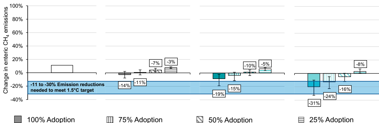
Fig. 3. Projected change in enteric methane ( \text{CH}_4 ) emissions between 2012 and 2030 without mitigation strategy under BAU and modeled mitigation scenarios (Product Based: adoption of one strategy that reduces product-based \text{CH}_4 emissions; Absolute: adoption of one strategy that reduces absolute \text{CH}_4 emissions; and Product Based & Absolute: adoption of one strategy that reduces product-based \text{CH}_4 emissions and one strategy that reduces absolute \text{CH}_4 emissions) for enteric \text{CH}_4 emission changes globally (A), in the African region (B), and in the European region (C). Error bars represent the average mitigation effect of the least and most effective mitigation strategy. Numbers in squares indicate the percentage of change from BAU.
