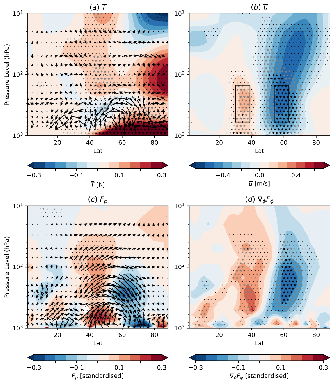
Fig. 3 Zonal mean response. Latitude-height cross sections of the multi-model ensemble mean zonally averaged DJF response of a temperature ( \bar{T} , colours, K, where the overbar denotes the zonal average) and transformed Eulerian mean (TEM, Methods) circulation (arrows), b zonal wind ( \bar{u} , \text{ms}^{-1} ), and c upward Eliassen-Palm (EP) flux ( F_p , colours, standard deviations) and EP flux vectors (arrows representing F_\phi and F_p ), d divergence of northward EP flux ( \nabla_\phi F_\phi , standard deviations). Stippling as in Fig. 1. To aid visualisation the TEM circulation and EP fluxes are standardised by dividing by the internal variability of the present-day simulations (Methods).
