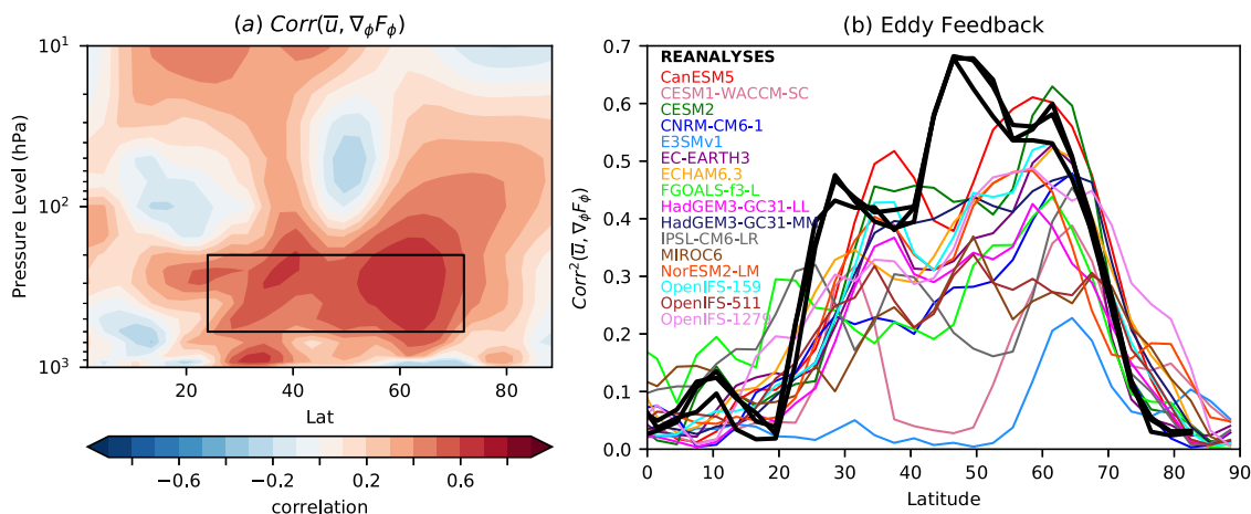
Fig. 6 Eddy feedback. a Latitude-height cross section of the multi-model mean local correlation between DJF \bar{u} and \nabla_\phi F_\phi . Correlations are computed across ensemble members for the present day simulation for each model separately, and then averaged to make the multi-model mean. b Fraction of mid-upper troposphere zonal wind variance explained by \nabla_\phi F_\phi as a function of latitude (the square of the local correlations in a averaged over 600 to 200 hPa) for each of the models (coloured curves) and in the reanalyses (black curves). Reanalyses values are computed from interannual time series over the period 1979–2016 inclusive. The eddy feedback parameter ( M ) is computed as the average over latitudes 25–72°N (shown by the box in a ).
