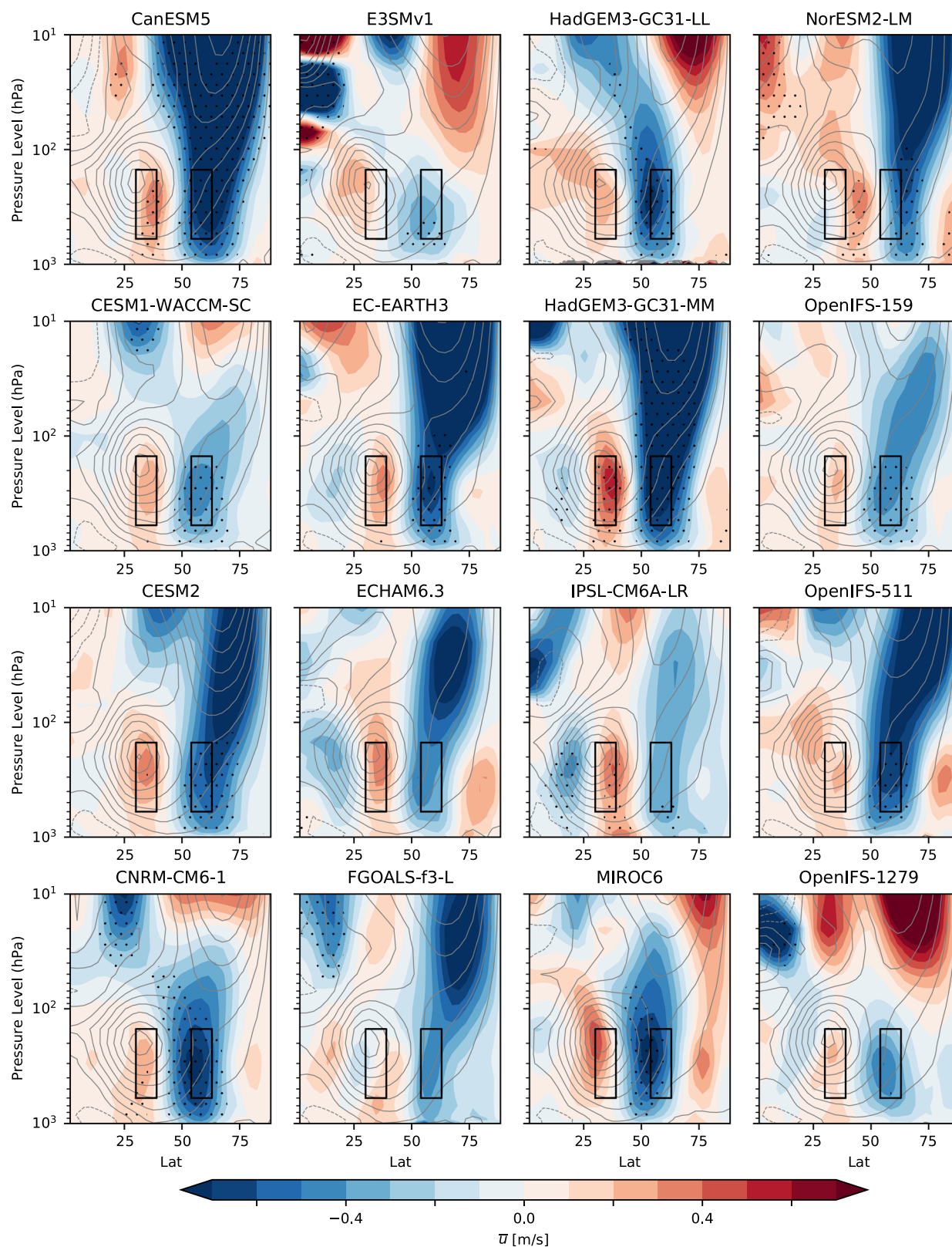
Fig. 2 Consistent tropospheric response to Arctic sea ice loss. Zonally averaged DJF zonal wind response ( \bar{u} , \text{ms}^{-1} , where the overbar denotes the zonal average) plotted as a function of latitude ( ^{\circ}\text{N} ) and height (pressure) for the ensemble mean of each of the models. The boxes show the regions used to compute the zonal wind response index (ZWRI). Stippling indicates where the ensemble mean response is significant (95% confidence interval). Contours show the climatological zonal mean winds (contour interval 5 \text{ ms}^{-1} with negative contours dotted).
