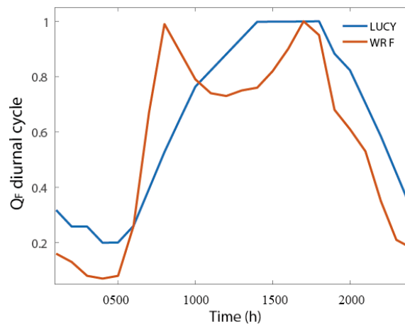
Figure 2: Normalized maximum anthropogenic heat flux diurnal cycle on all days. LUCY: Large-Scale Urban Consumption of Energy Model.
