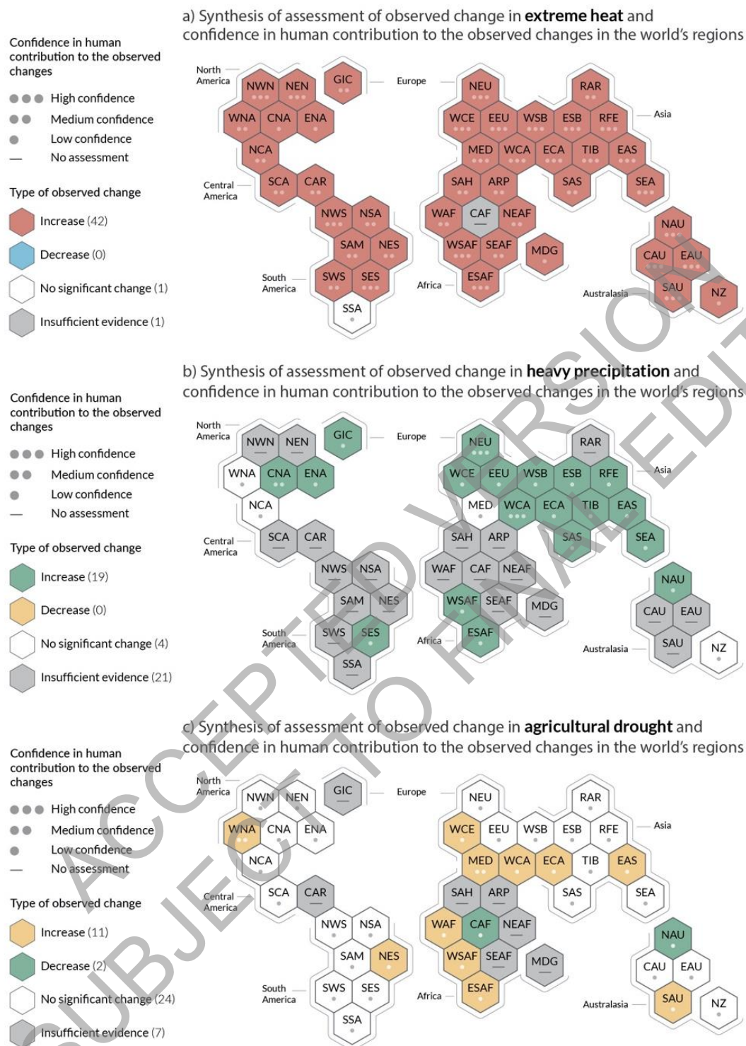
Box TS.10, Figure 1: Synthesis of assessed observed changes and human influence of hot extremes (panel a), heavy precipitation (panel b) and agricultural and ecological drought (panel c) for the IPCC AR6 regions (displayed as hexagons). The colours in each panel represent the four outcomes of the assessment on the observed changes: In Panel a): red – at least medium confidence in an observed increase in hot extremes; blue – at least medium confidence in an observed decrease in hot extremes; white – no significant change in hot extremes is observed for
