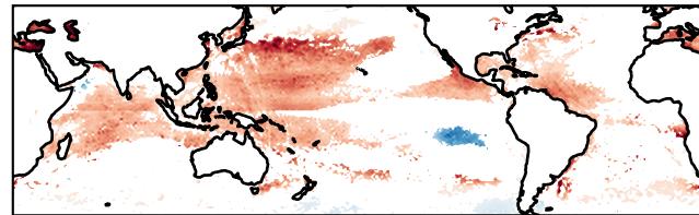
d Modified Carnot efficiency [unitless fraction decade ^{-1} ]
