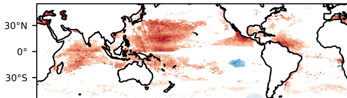
e Genesis potential [ 10^4 \times \text{m}^{-2} \text{ s}^{-1} \text{ decade}^{-1} ]
