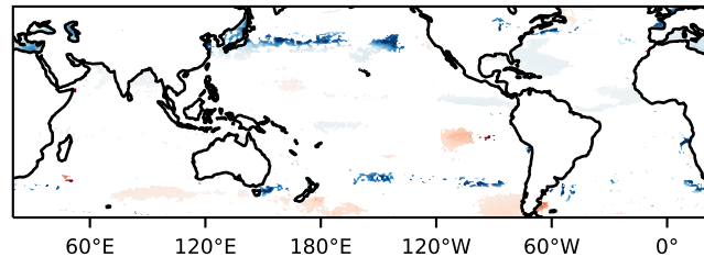
f Tropical cyclone outflow temperature [ ^{\circ}\text{C decade}^{-1} ]
