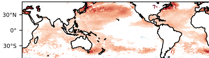
c Air-sea thermodynamic disequilibrium [ 10^2 \times \text{J kg}^{-1} \text{ decade}^{-1} ]
