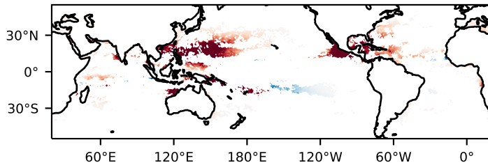
e Genesis potential [ 10^4 \times \text{m}^{-2} \text{ s}^{-1} \text{ decade}^{-1} ]
