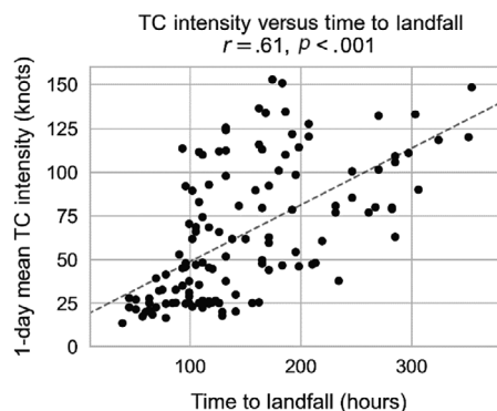
FIGURE 8 TC intensity before landfall compared to time from TC cyclogenesis until landfall in Luzon. The dashed line shows the least-squares regression slope for each relationship. The Pearson correlation coefficient ( r ) and p value ( p ) are listed above each plot
