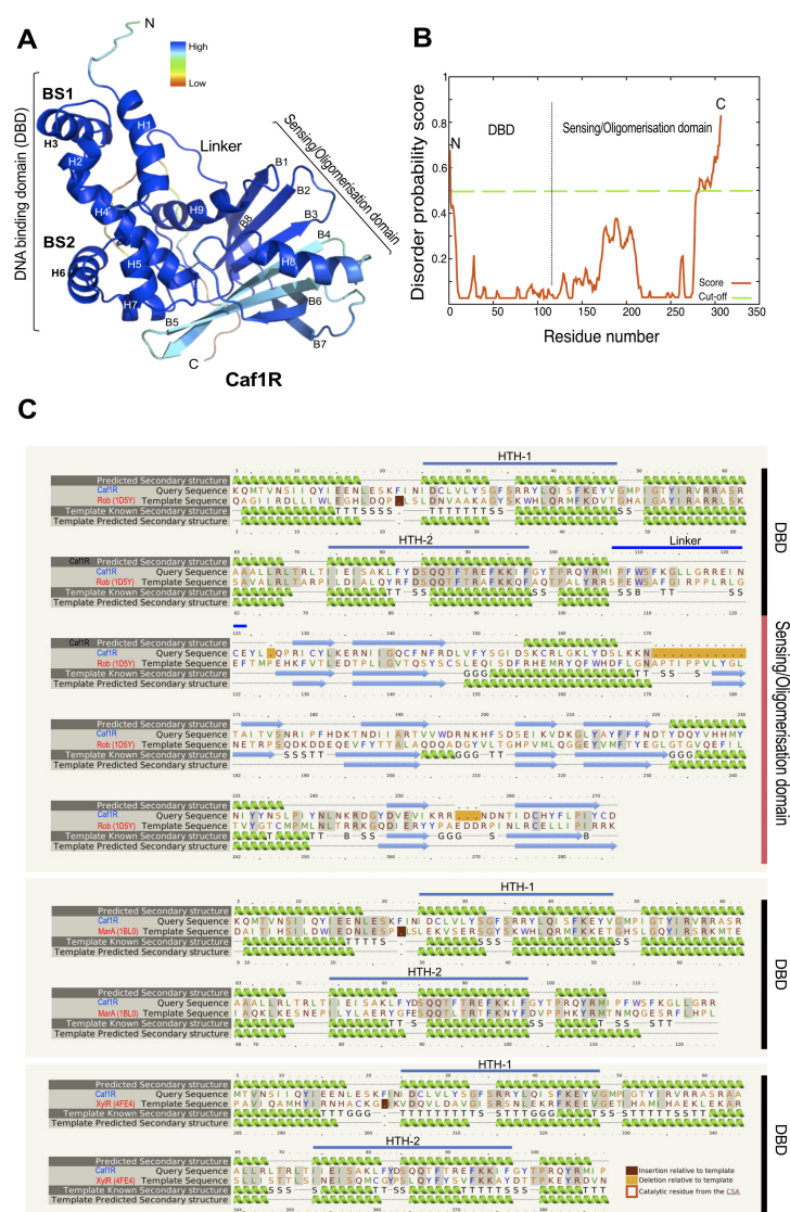
Figure 1. Caf1R modelled structure and its homology with E. coli Rob, MarA and XylR. (A) Int-FOLD3.0 [49] predicted model of the full-length Caf1R on Rob protein template (PDB 1D5Y). Quality of prediction is indicated by the \beta -factor colour intensity and its \geq 70\% non-redundancy, computed by IntFOLD3.0. Predicted DNA-binding domain (DBD) at the N-terminus composed of seven alpha helices (H1–H7), connected by an unstructured linker to the putative sensing/oligomerisation domain at the C-terminus, comprised of H8–H9 and eight \beta -strands (B1–B8). (B) Disorder prediction plot (per residue) of the modelled structure, reinforces reliability of the Caf1R model. MacPyMOL1.3 was used to visualise and generate the ribbon diagrams of modelled Caf1R. (C) Phyre2 [50] predicted secondary structures alignment of the full-length native Caf1R (query) with the closest A/X family structural homologues, Rob (PDB 1D5Y), MarA (PDB 1BL0) and XylR (PDB 4FE4) as indicated. The helix-turn-helix (HTH) motifs of Caf1R-DBD, HTH-1 (H2–H3) and HTH-2 (H5–H6) are displayed with a thick blue line over respective helices. Amino acids highlighted in grey indicate aa identity of corresponding protein template with Caf1R: Rob (24%), MarA (34%) and XylR (35%). Seamless alignment of the Caf1R predicted secondary structures on the Rob template, confirms reliability of full-length Caf1R model.
