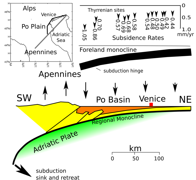
Figure 4. Geological setting of the Po Plain area with dominant tectonic features (adapted from Cuffaro et al., 2010).
